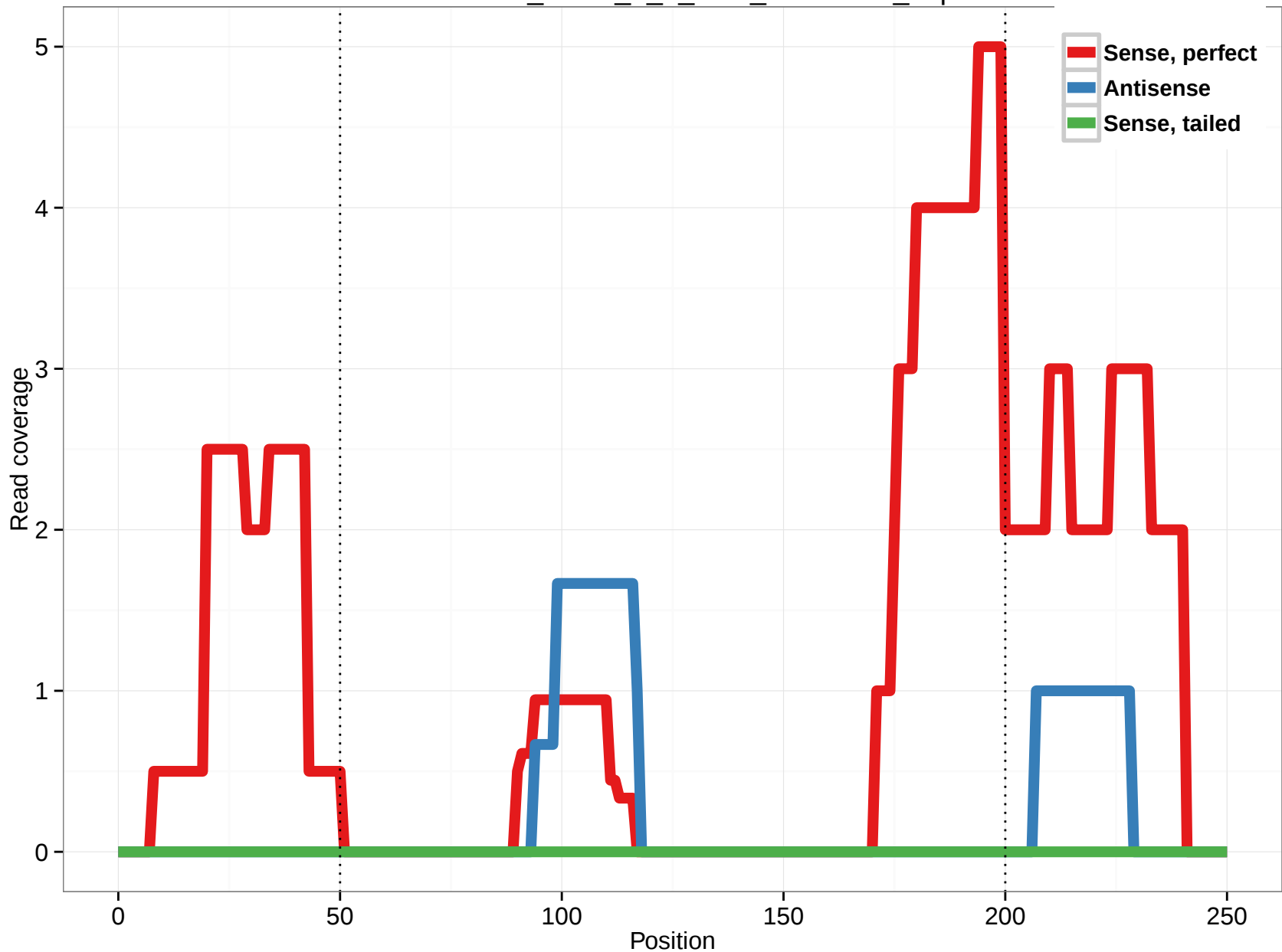
uc003tcv.1_intron_5_0_chr7_32591908_f.3p
