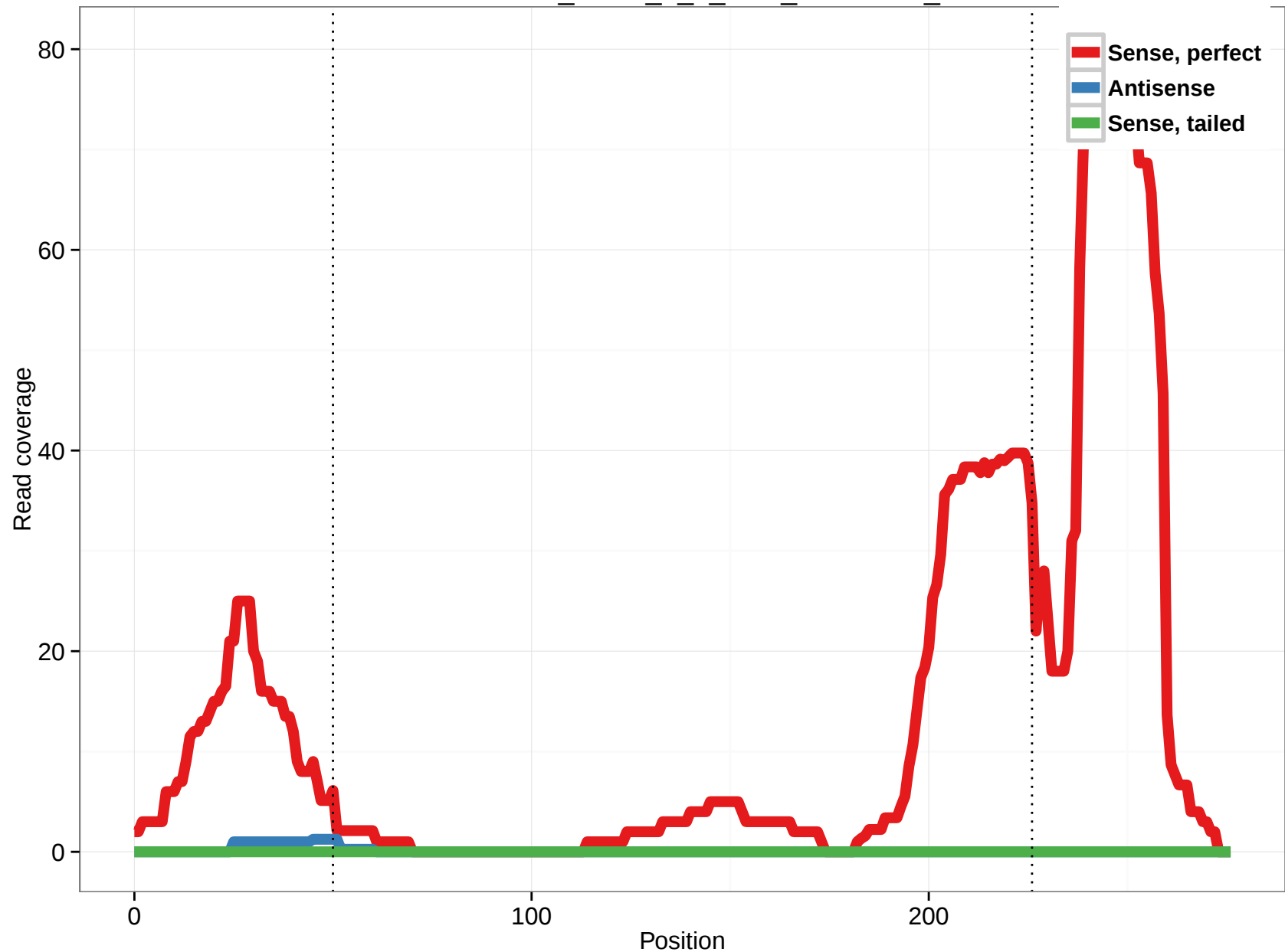
uc003swi.2_intron_0_0_chr7_23545189_r
