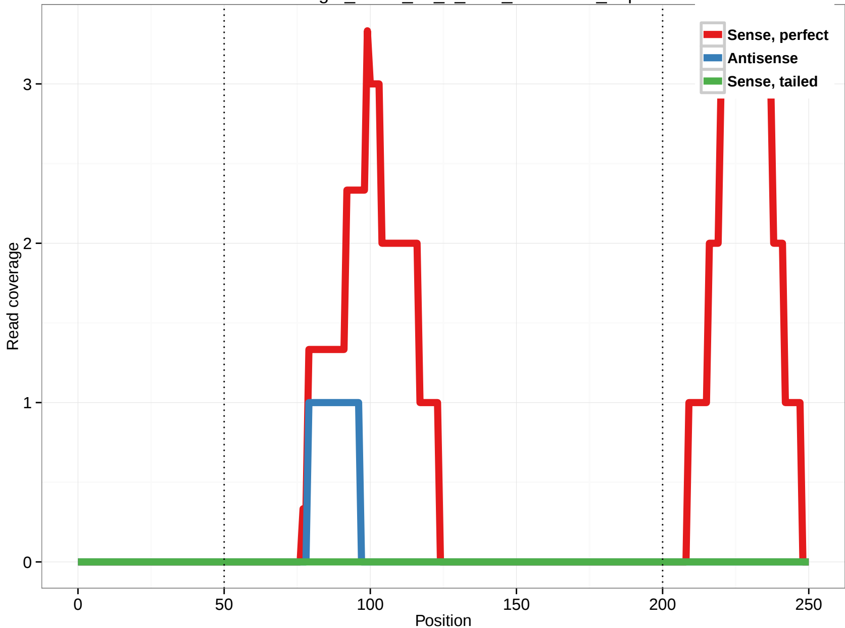
uc003svg.2_intron_24_0_chr7_22357657_r.3p
