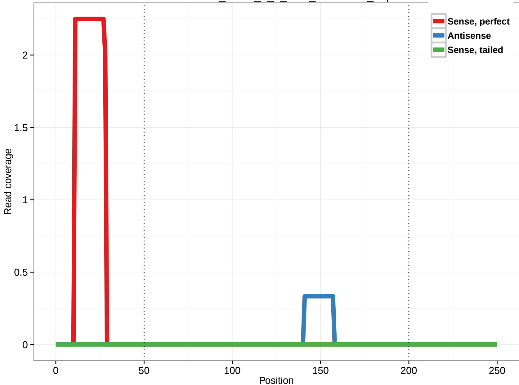
uc003sus.3_intron_5_0_chr7_20210402_r.3p
