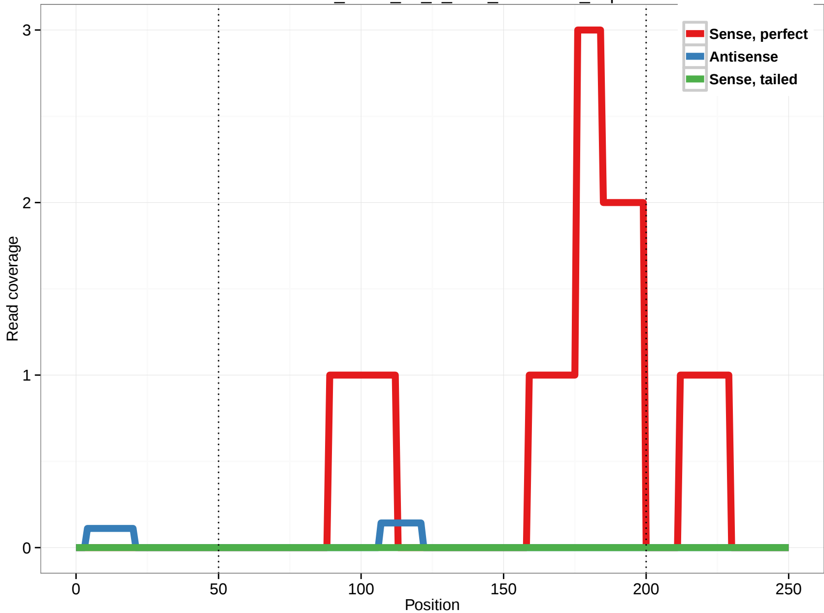
uc003srz.2_intron_16_0_chr7_11151095_f.3p
