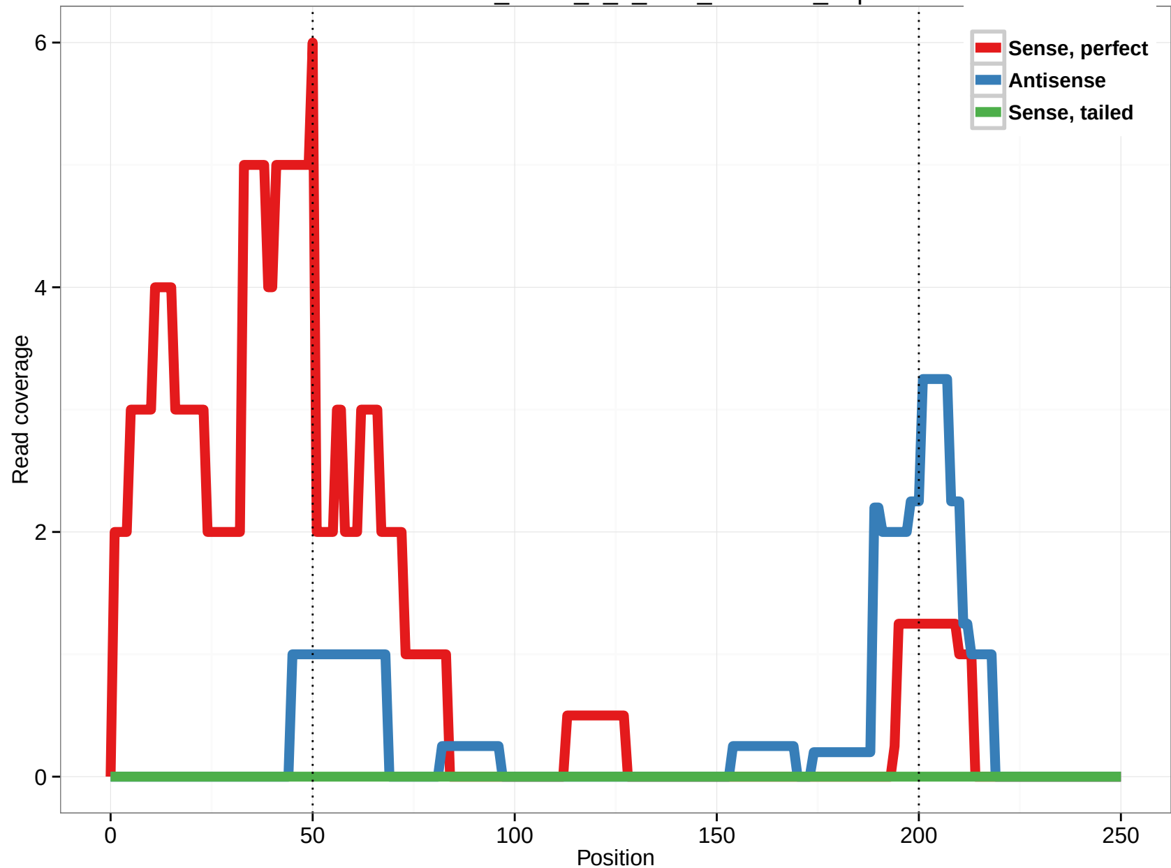
uc003son.3_intron_3_0_chr7_5545262_r.5p
