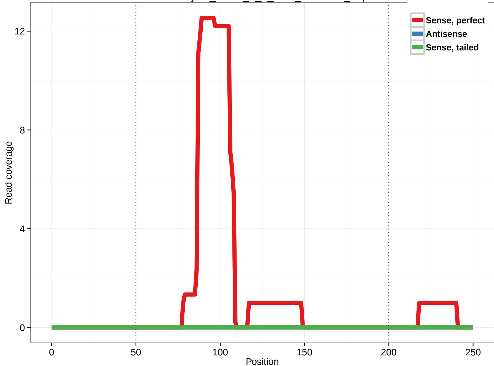
uc003sju.2_intron_3_0_chr7_1167023_r.3p
