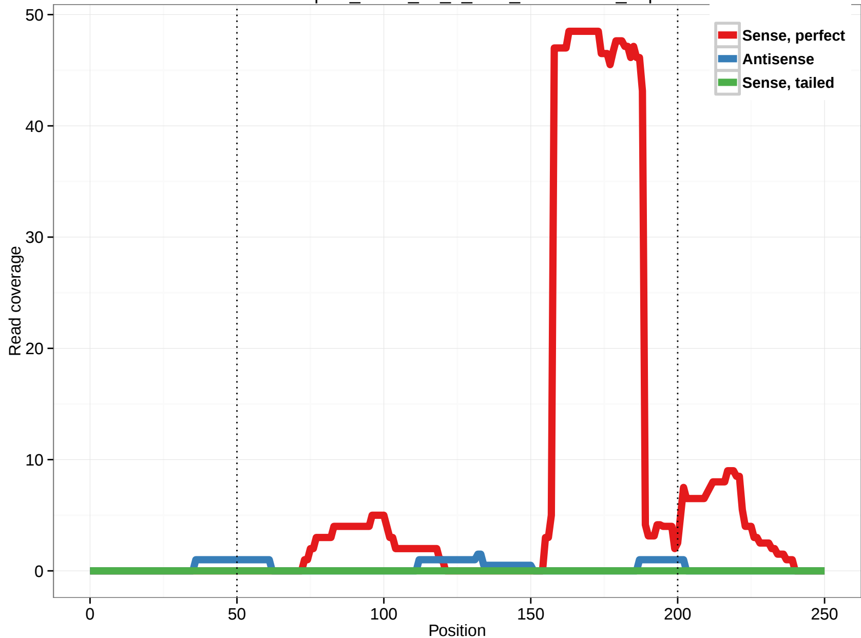
uc003qsr.2_intron_10_0_chr6_160209176_r.3p
