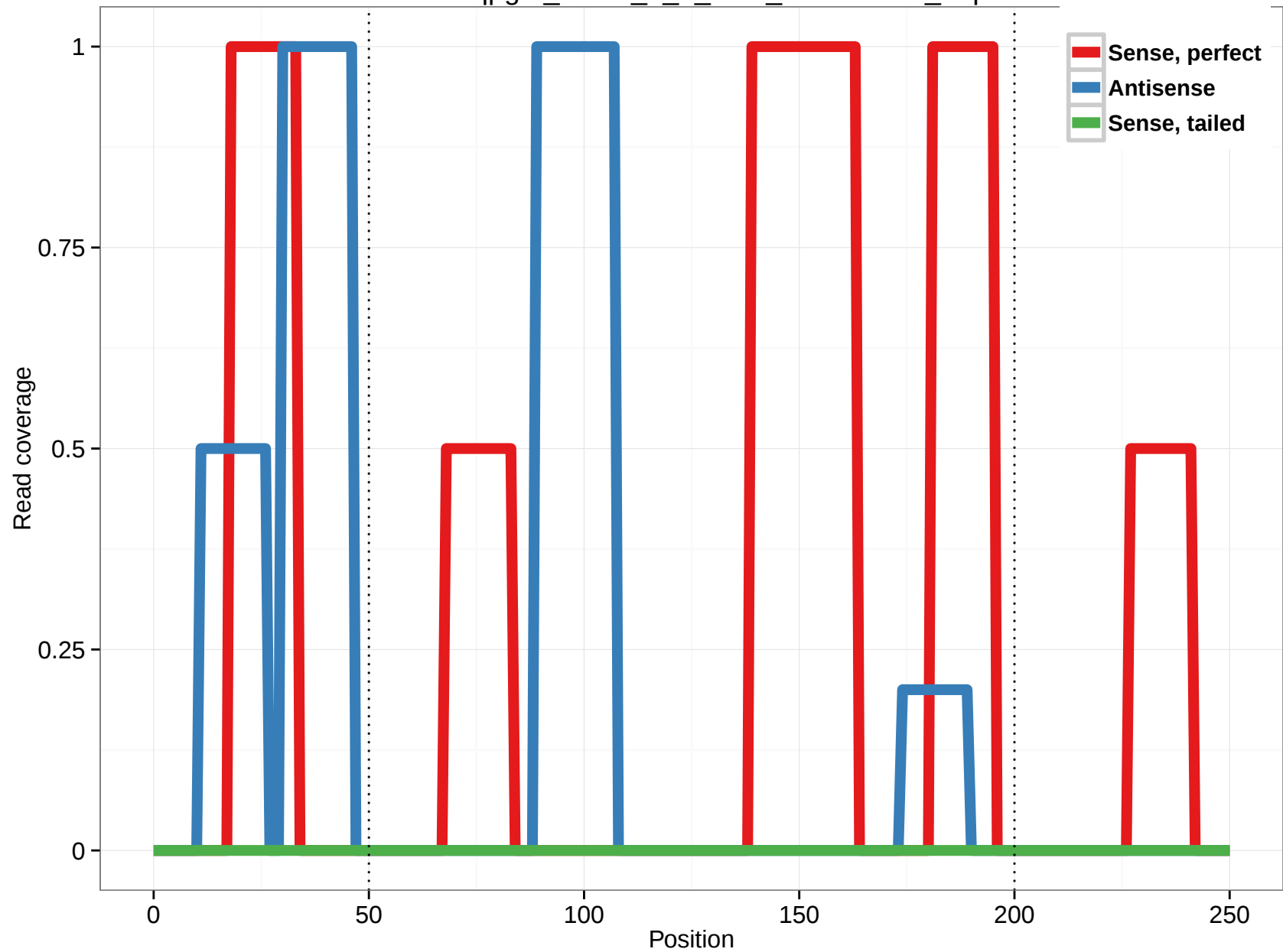
uc003qpg.2_intron_3_0_chr6_153296757_r.5p
