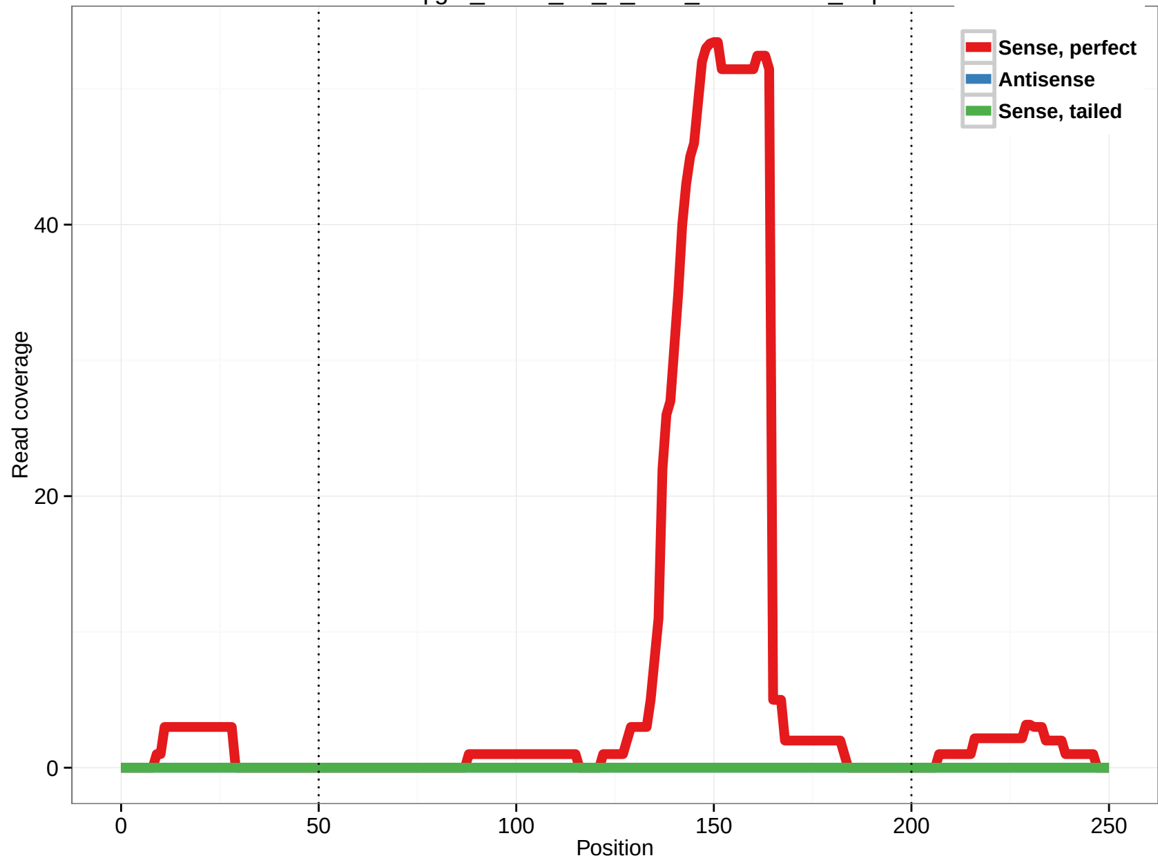
uc003qlg.1_intron_10_0_chr6_146248414_r.3p
