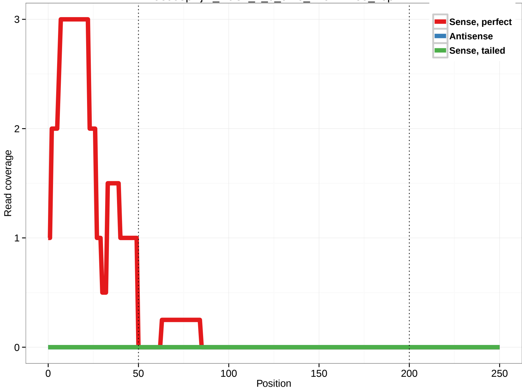
uc003pwj.2_intron_1_0_chr6_116427499_f.5p
