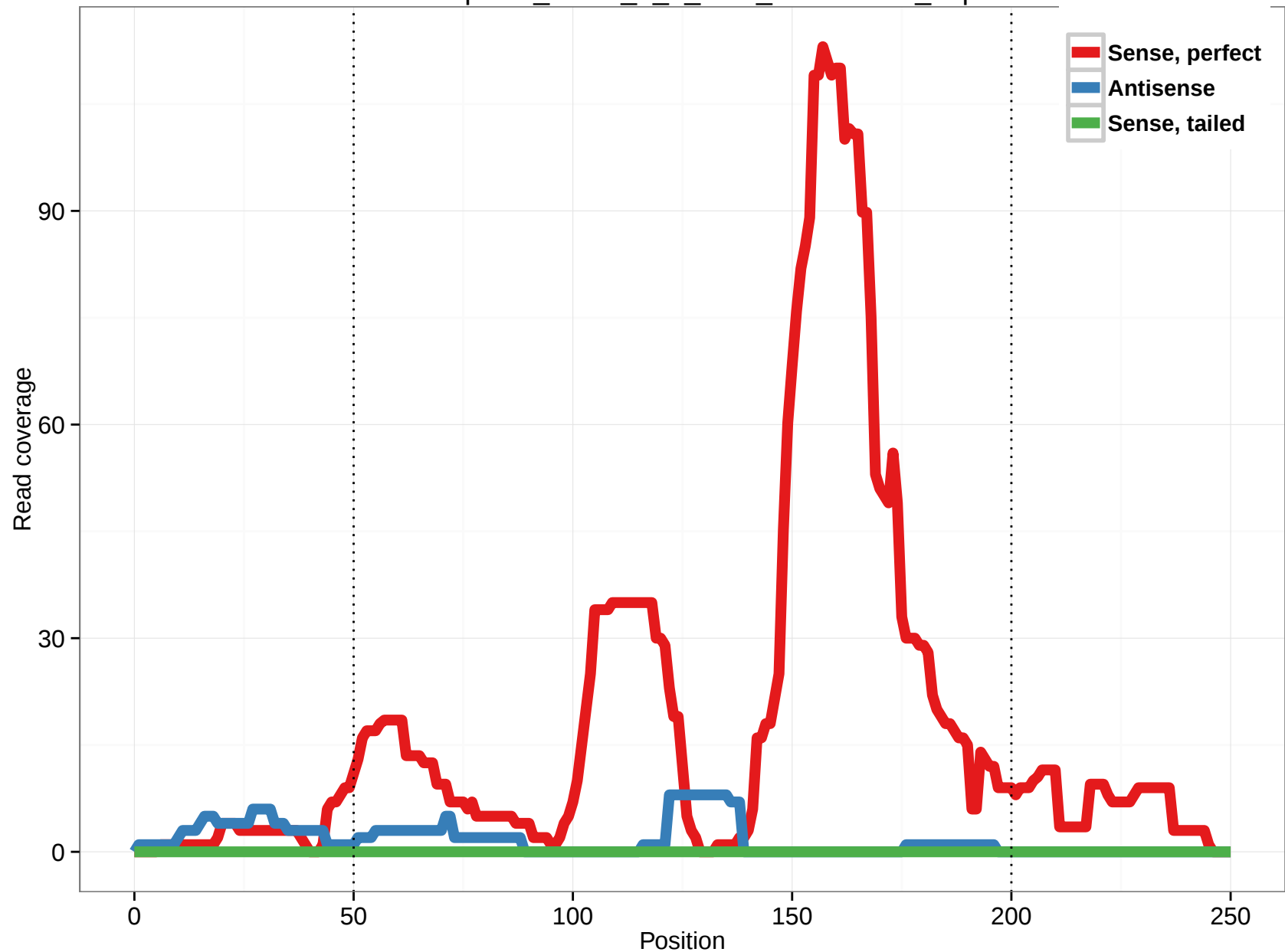
uc003pvb.2_intron_1_0_chr6_111805349_f.5p
