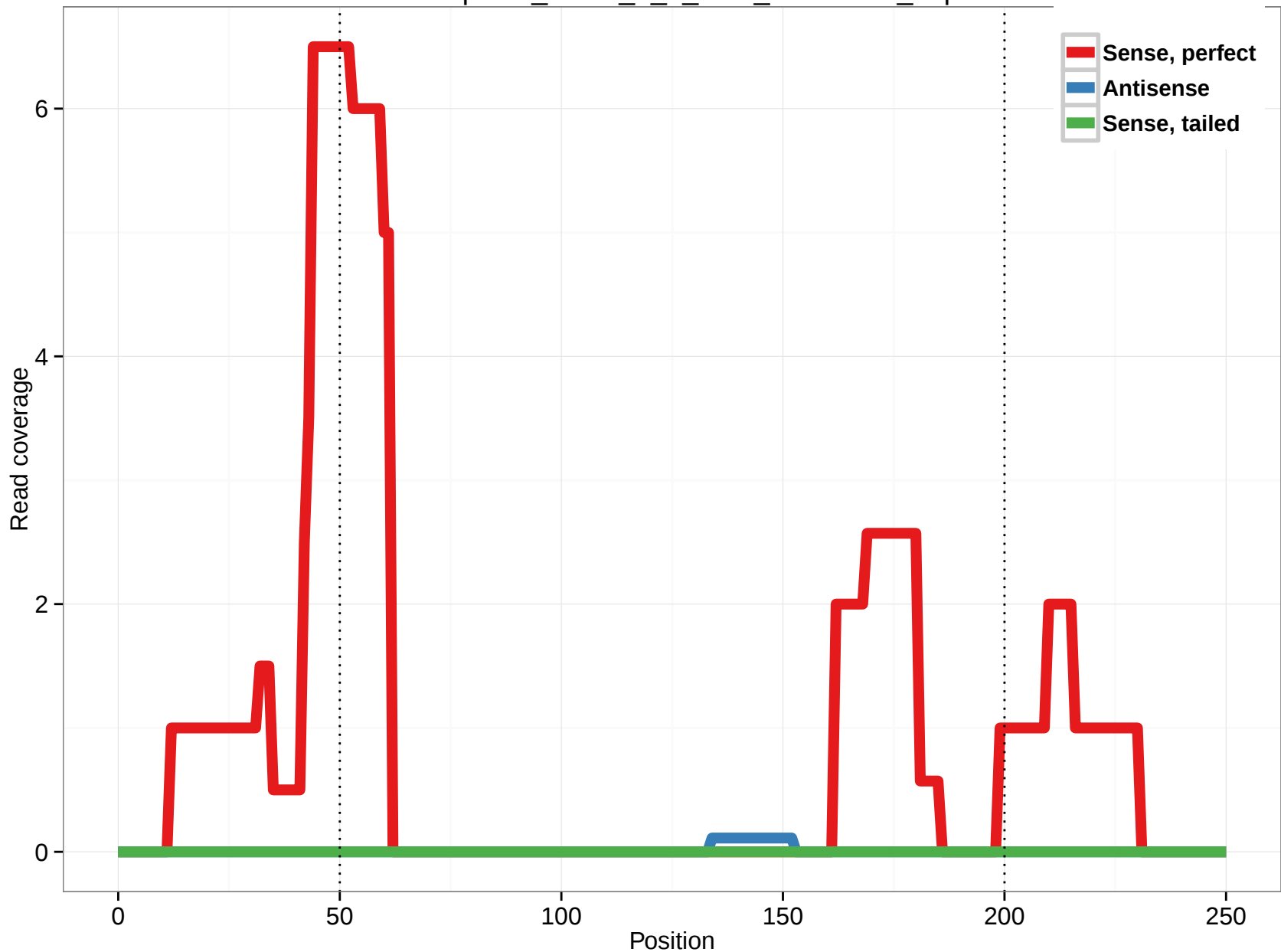
uc003pns.2_intron_2_0_chr6_90562954_f.3p
