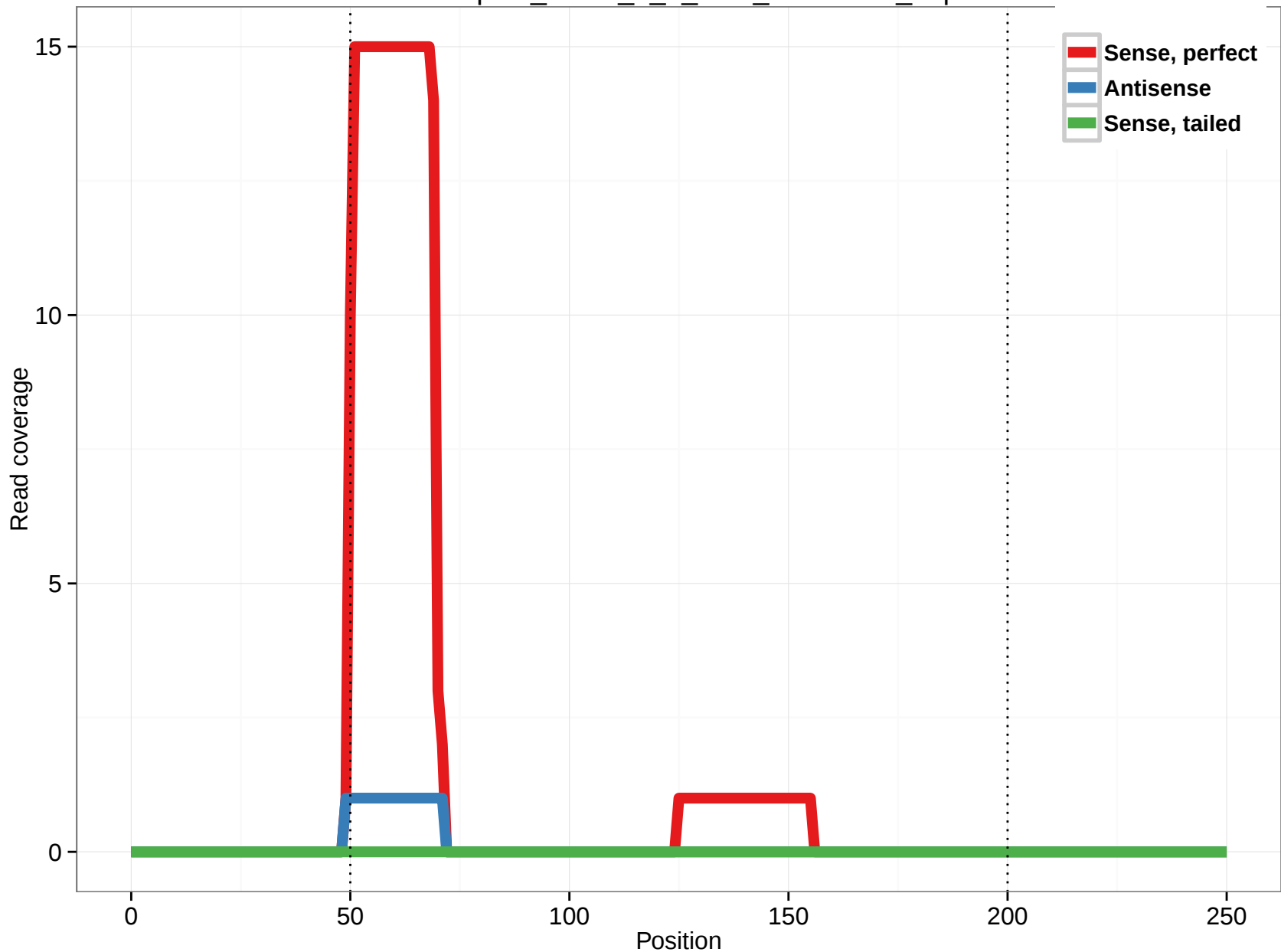
uc003plr.2_intron_4_0_chr6_88101596_f.5p
