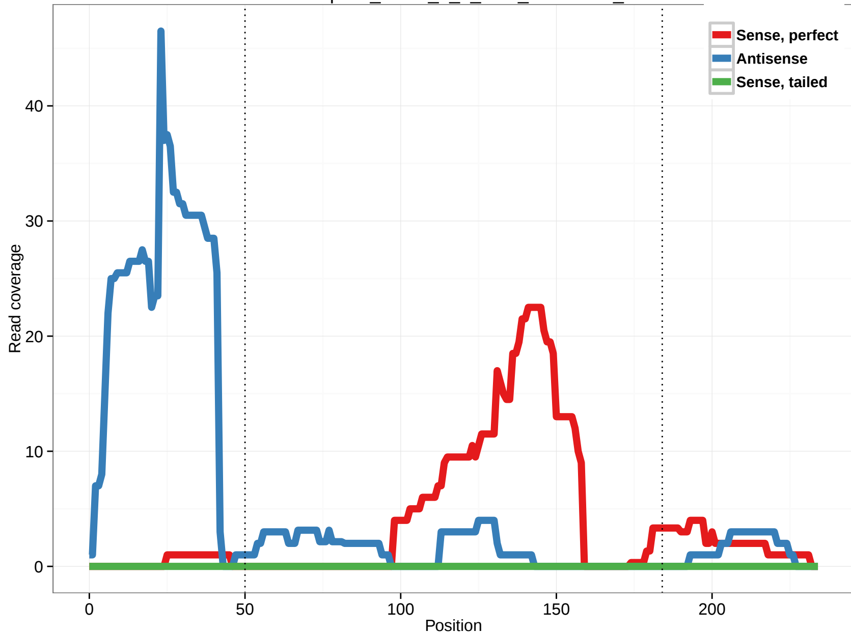
uc003piv.1_intron_0_0_chr6_79943645_f
