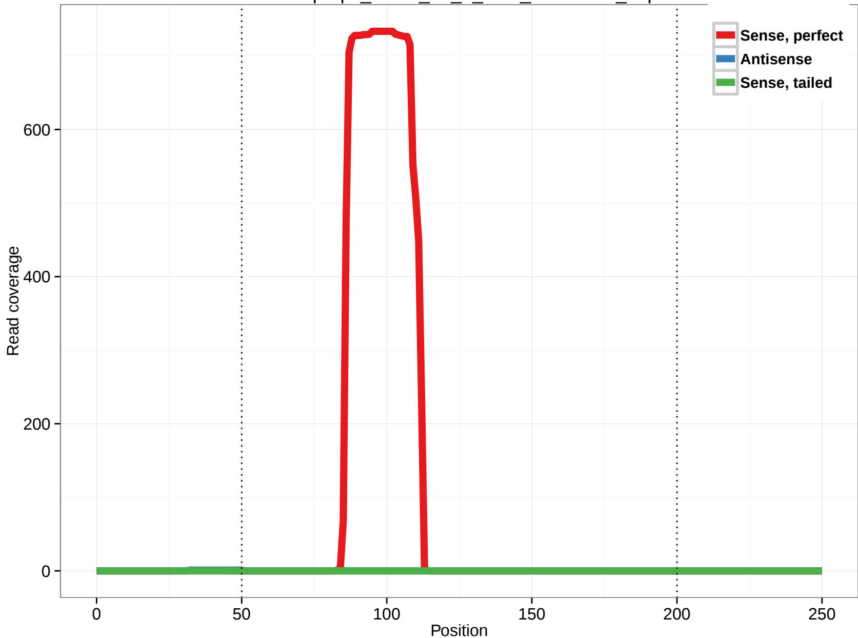
uc003phq.2_intron_23_0_chr6_74513025_f.3p
