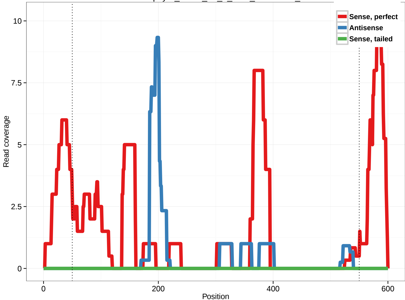
uc003pcy.3_intron_18_0_chr6_56357232_r
