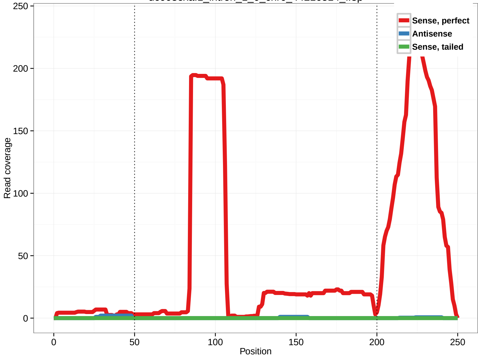
uc003oxa.1_intron_1_0_chr6_44216514_f.3p
