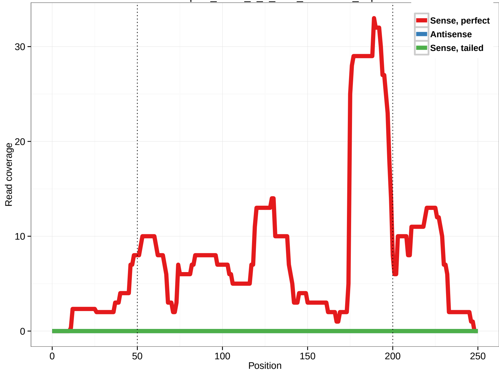
uc003ops.2_intron_0_0_chr6_41068918_f.5p
