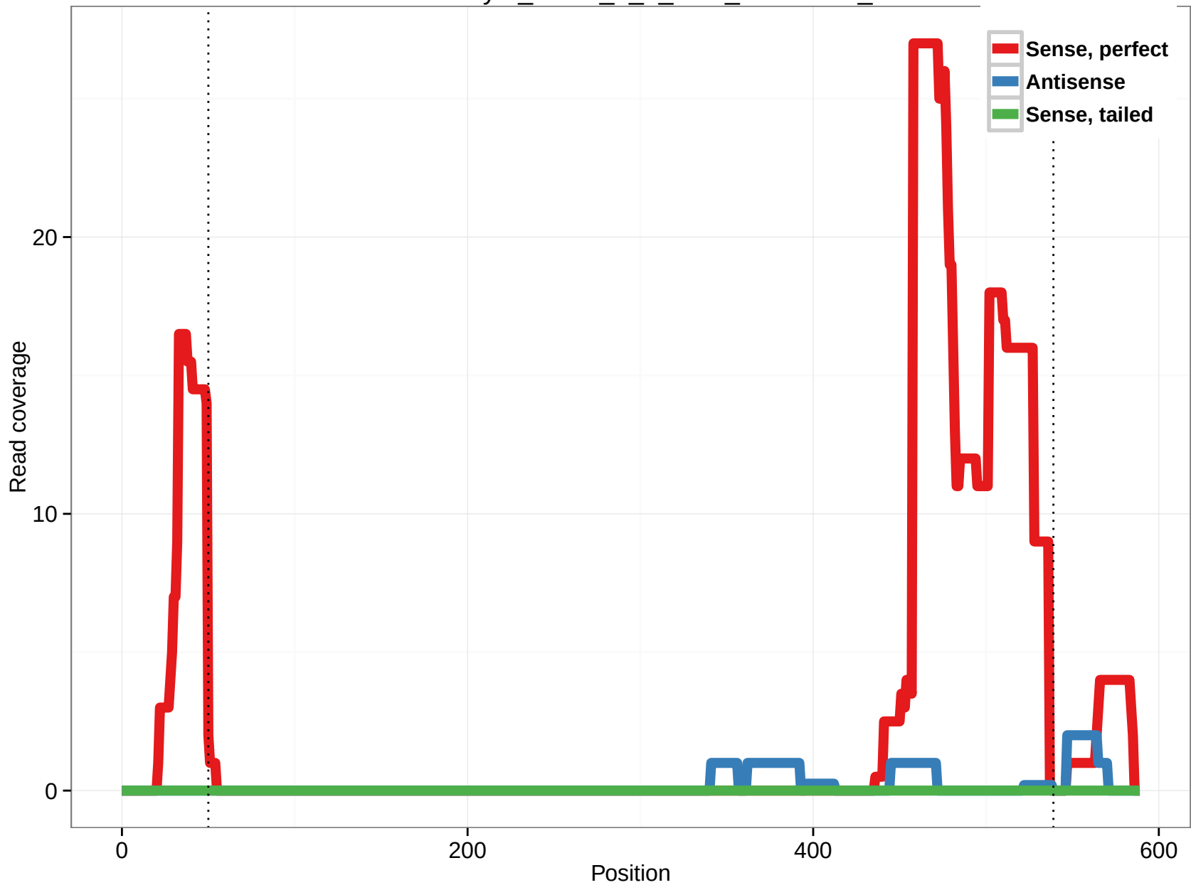
uc003oey.2_intron_1_0_chr6_33654297_f
