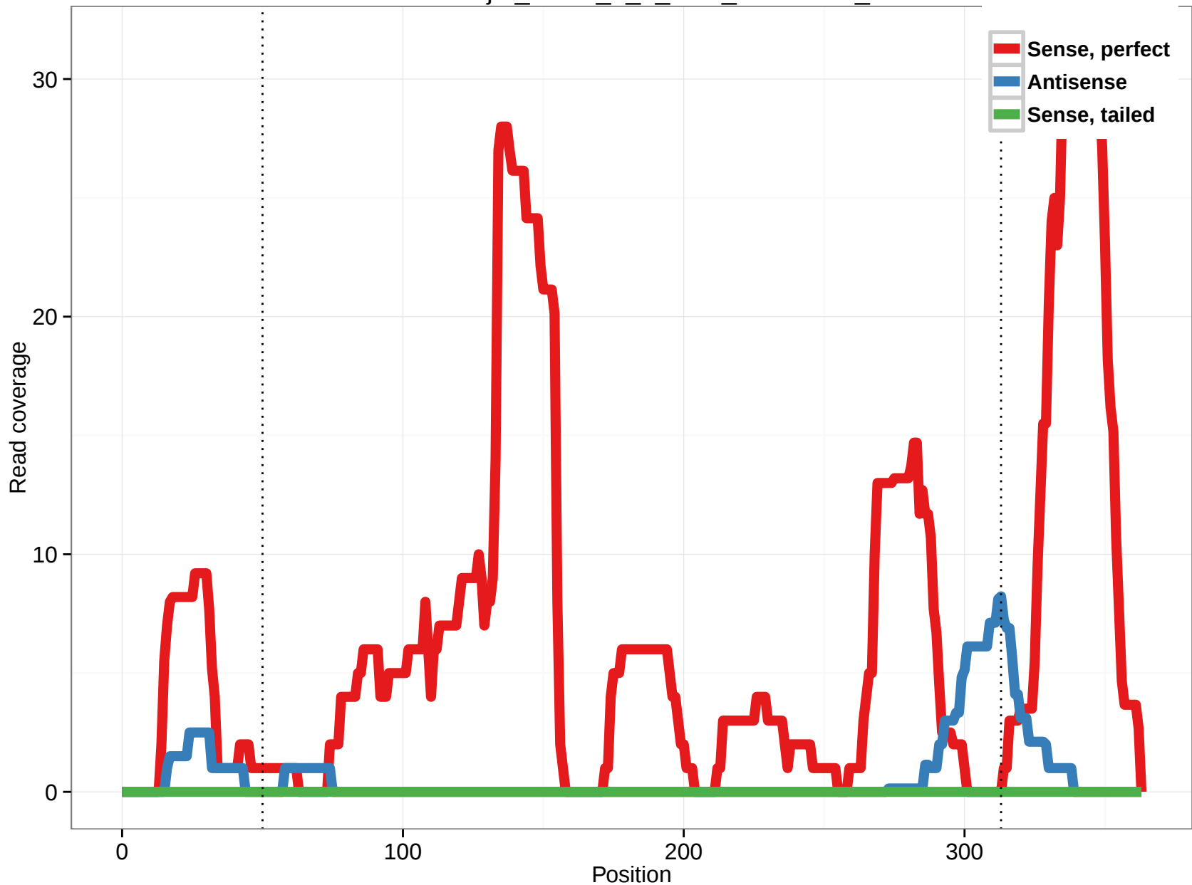
uc003oej.1_intron_4_0_chr6_33385473_r
