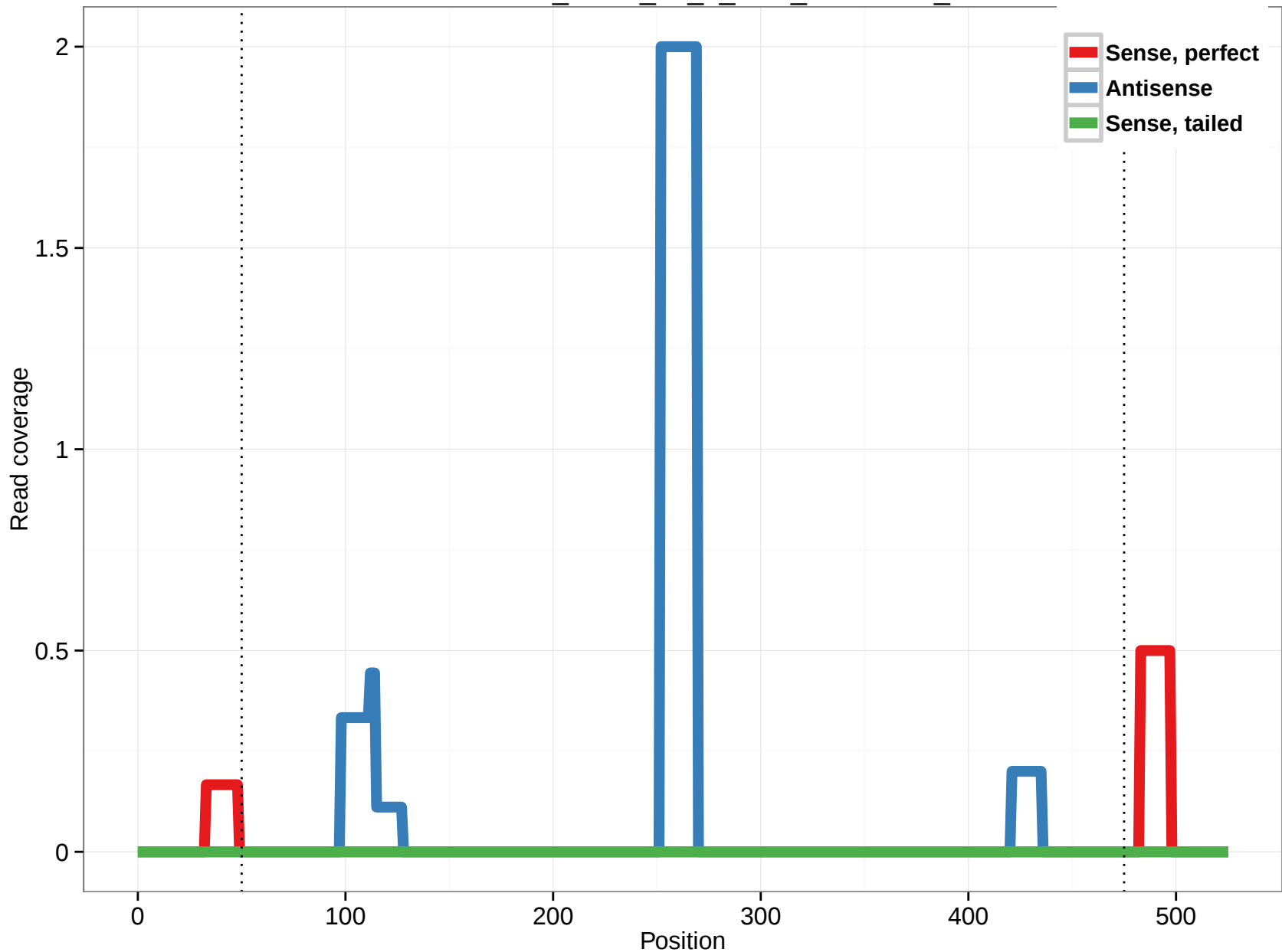
uc003ocx.1_intron_44_0_chr6_33145484_r
