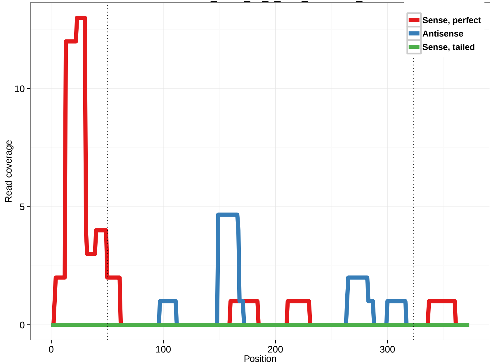
uc003nwt.1_intron_16_0_chr6_31727290_f
