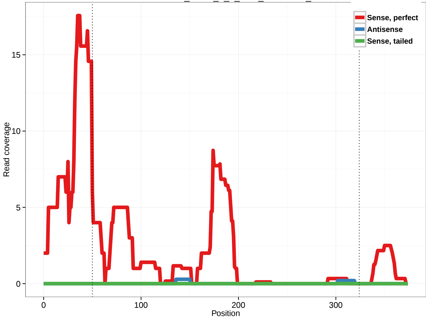
uc003ntk.1_intron_1_0_chr6_31378575_f
