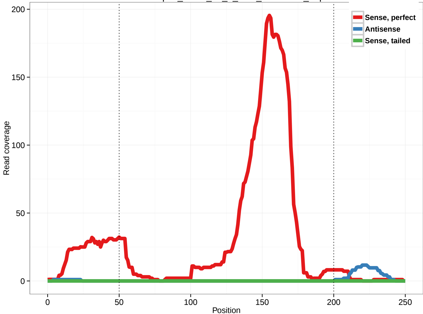
uc003nqn.1_intron_17_0_chr6_30577733_r.5p
