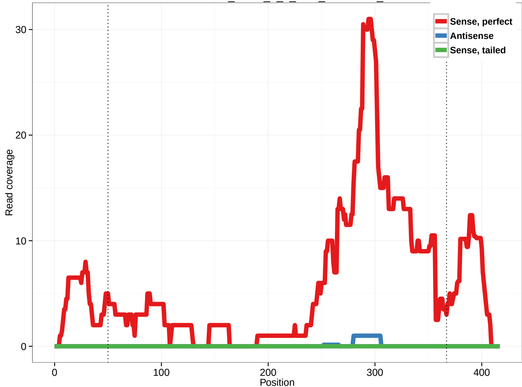
uc003mzr.2_intron_1_0_chr6_11135221_f
