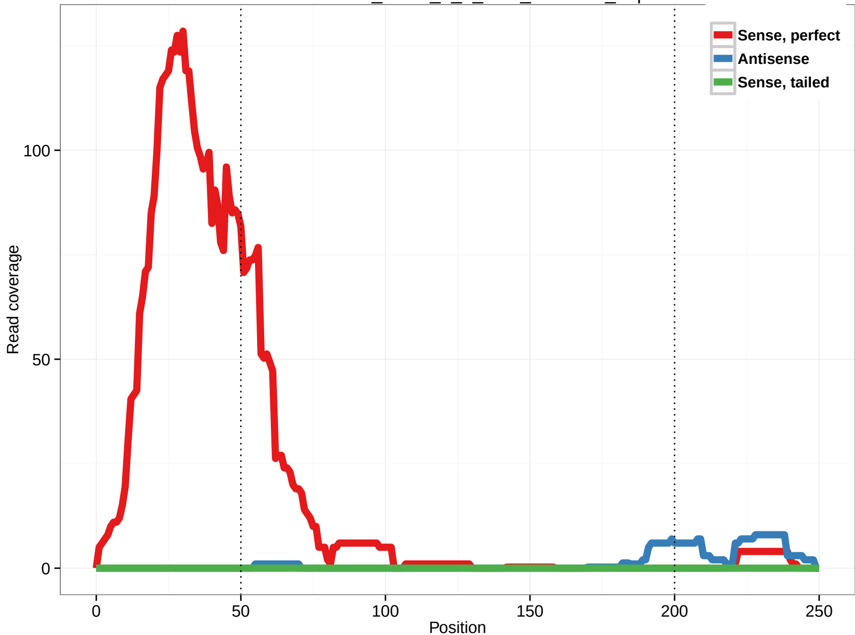
uc003mub.2_intron_5_0_chr6_2840829_r.5p
