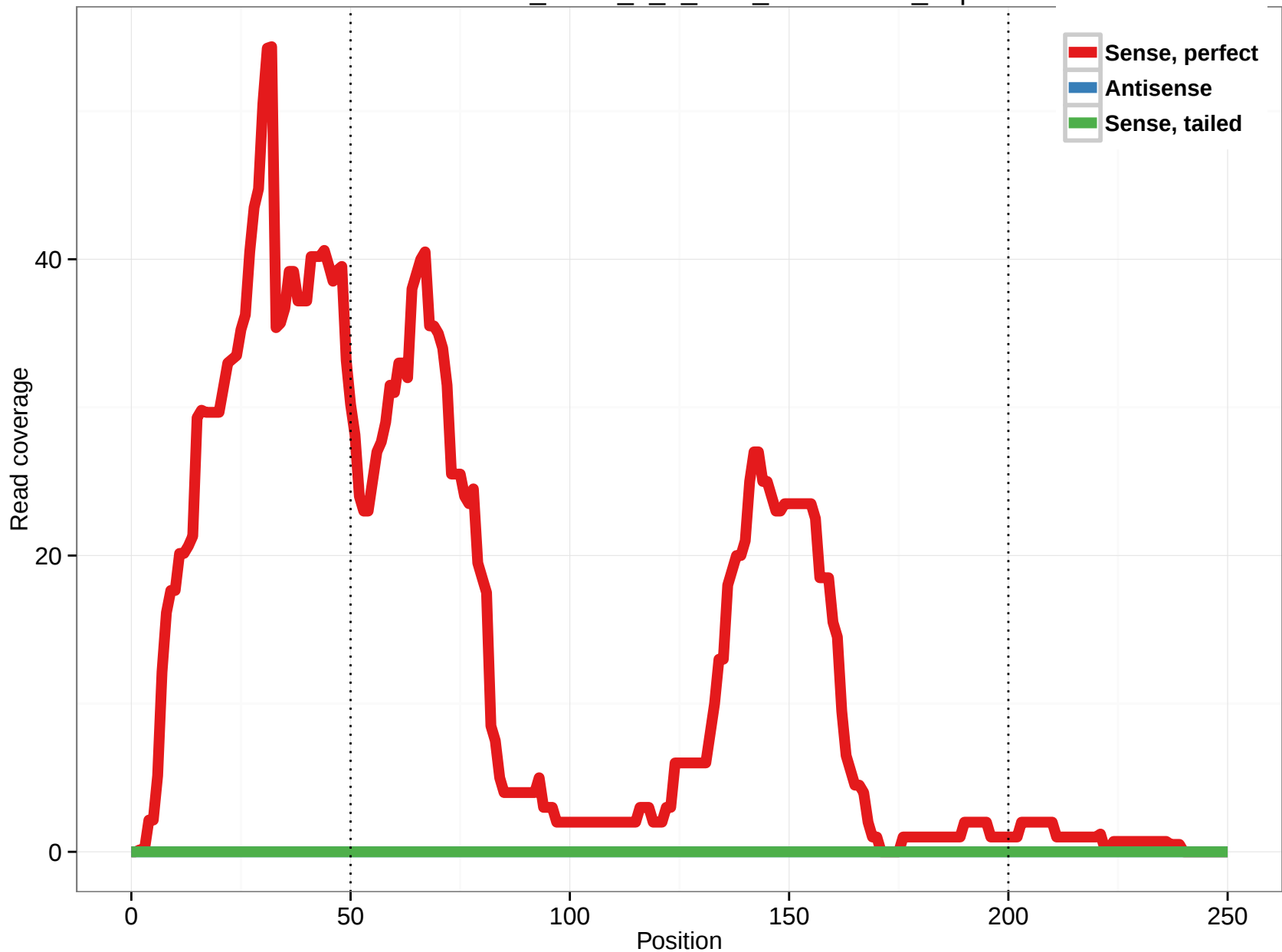
uc003mkf.3_intron_8_0_chr5_179045325_r.5p
