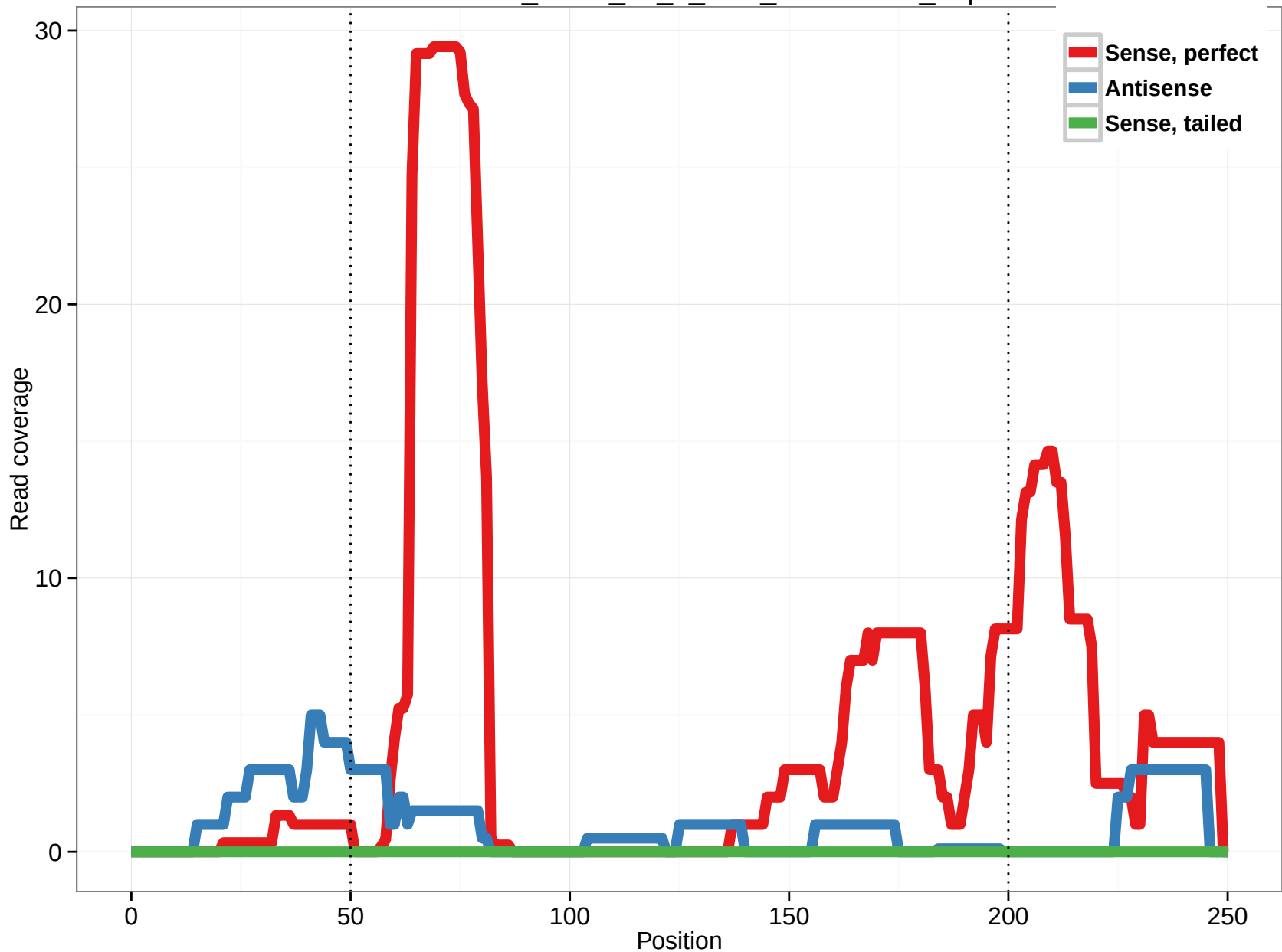
uc003miz.2_intron_11_0_chr5_177658525_r.5p
