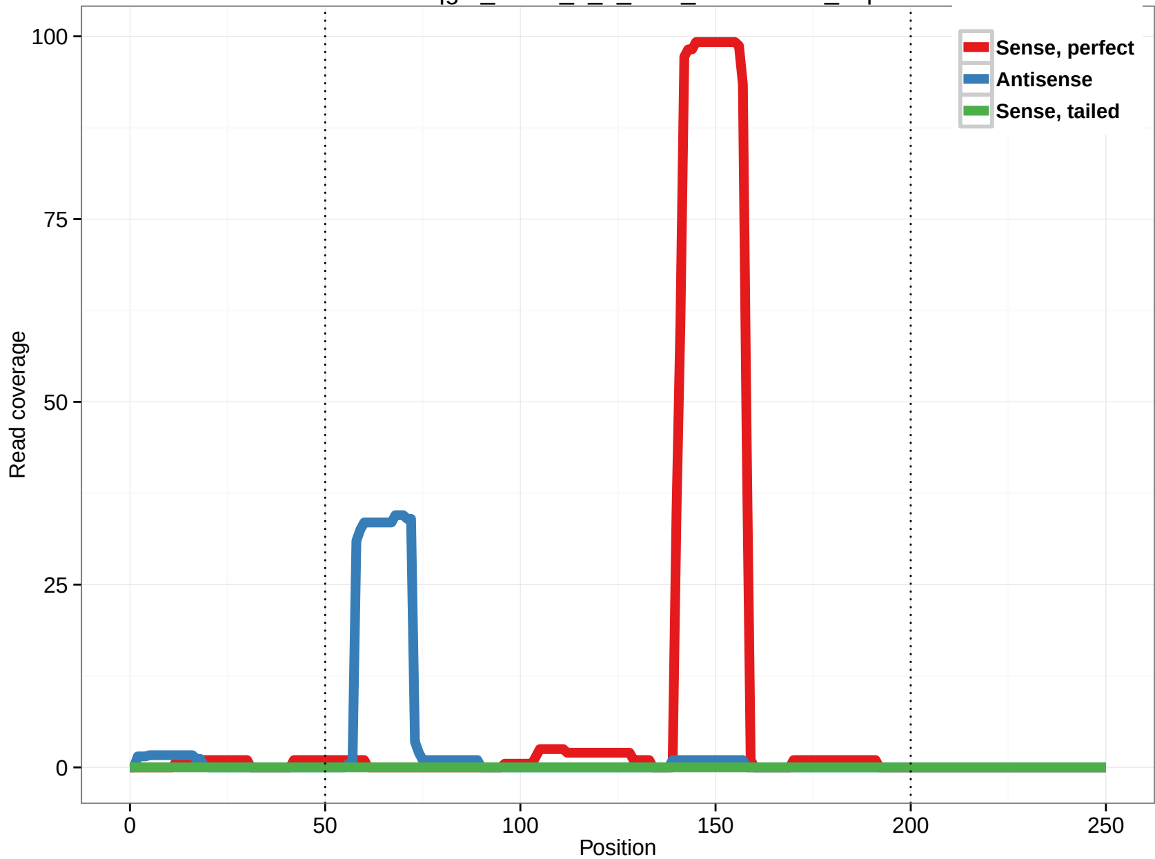
uc003lqg.3_intron_0_0_chr5_148651548_f.5p
