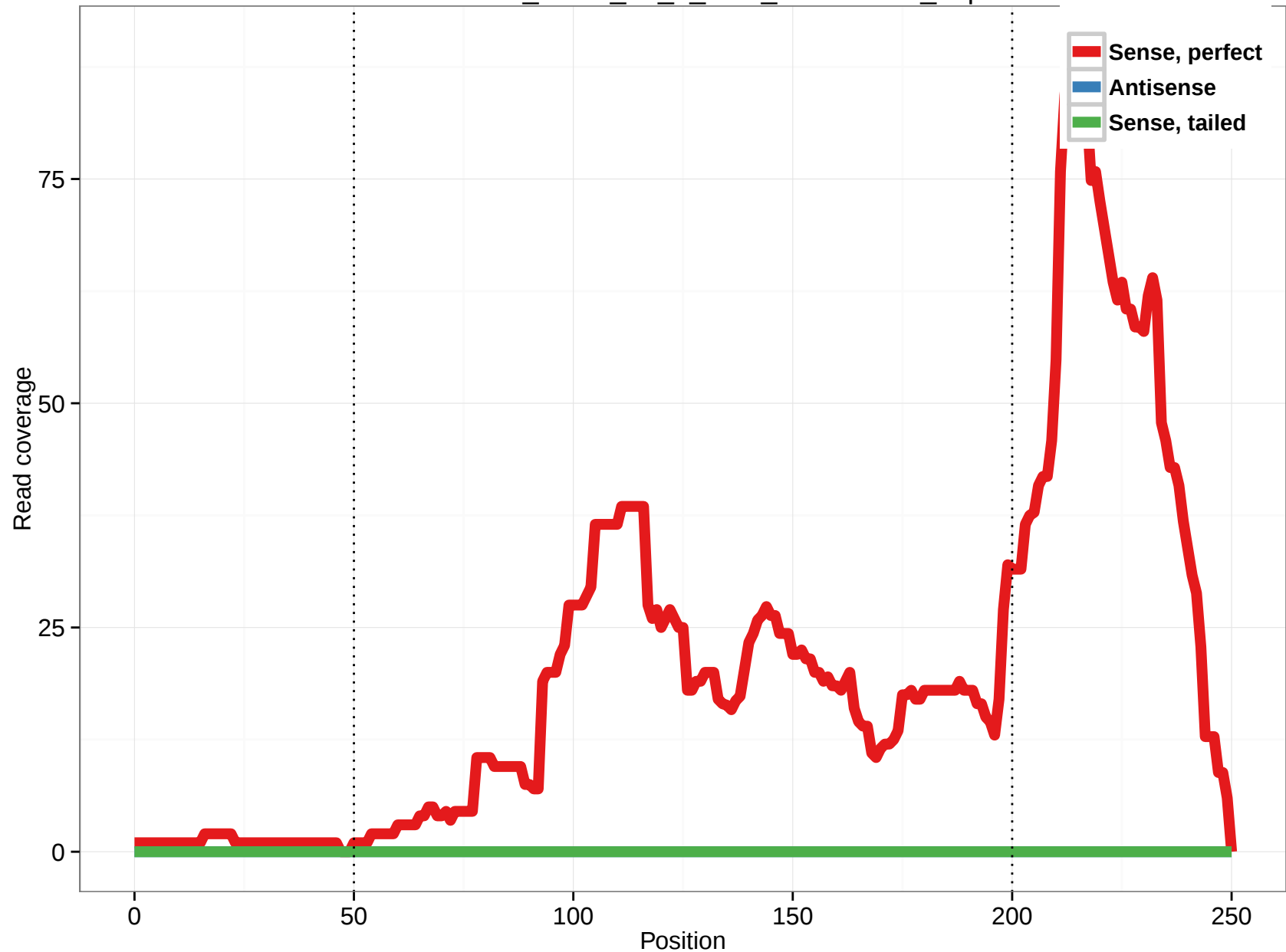
uc003ldu.2_intron_14_0_chr5_138658657_f.3p
