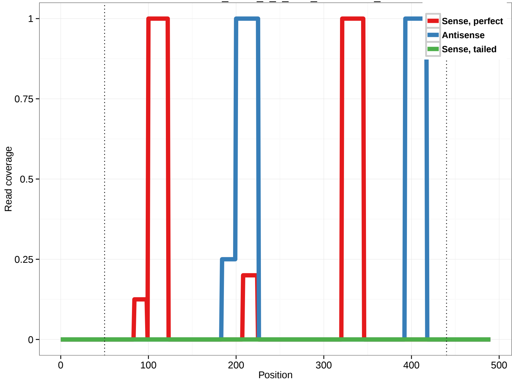
uc003lcn.2_intron_1_0_chr5_137589065_r
