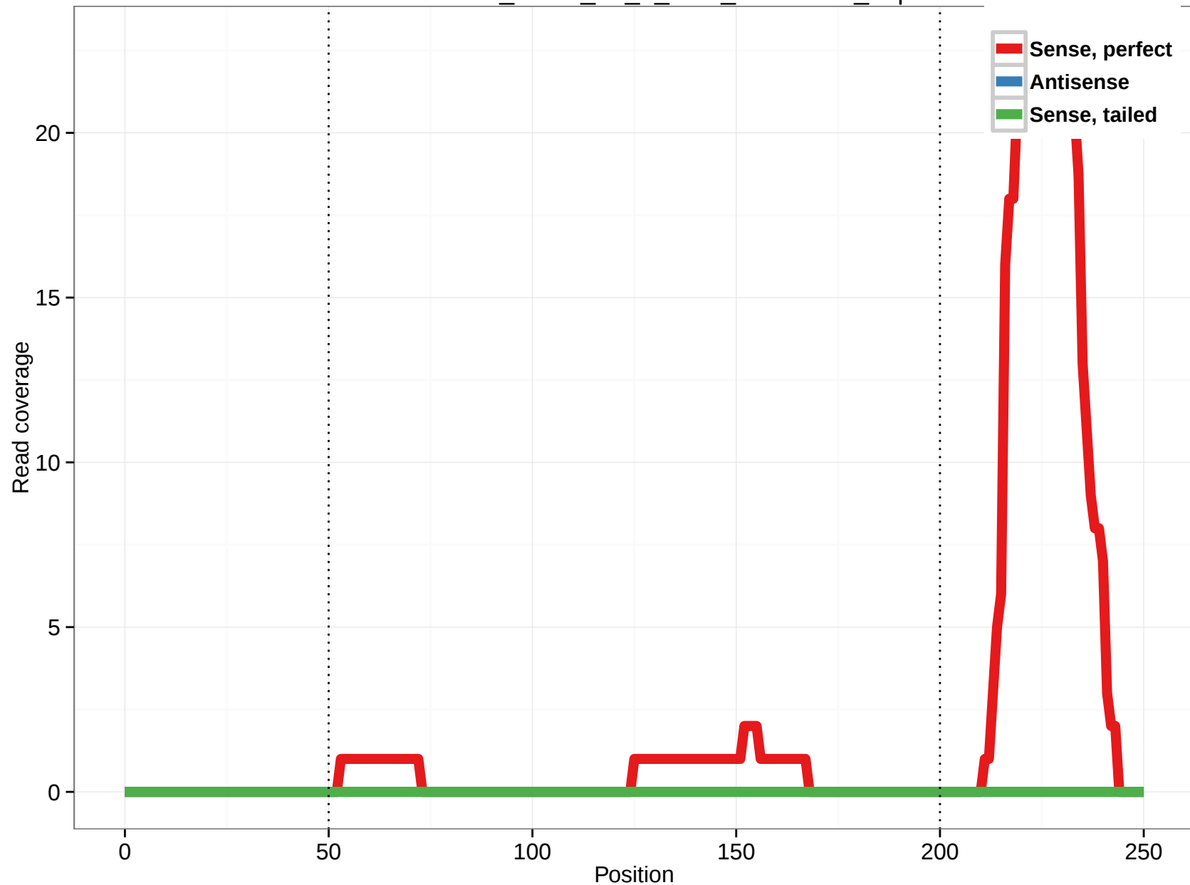
uc003kmv.1_intron_10_0_chr5_96342220_f.3p
