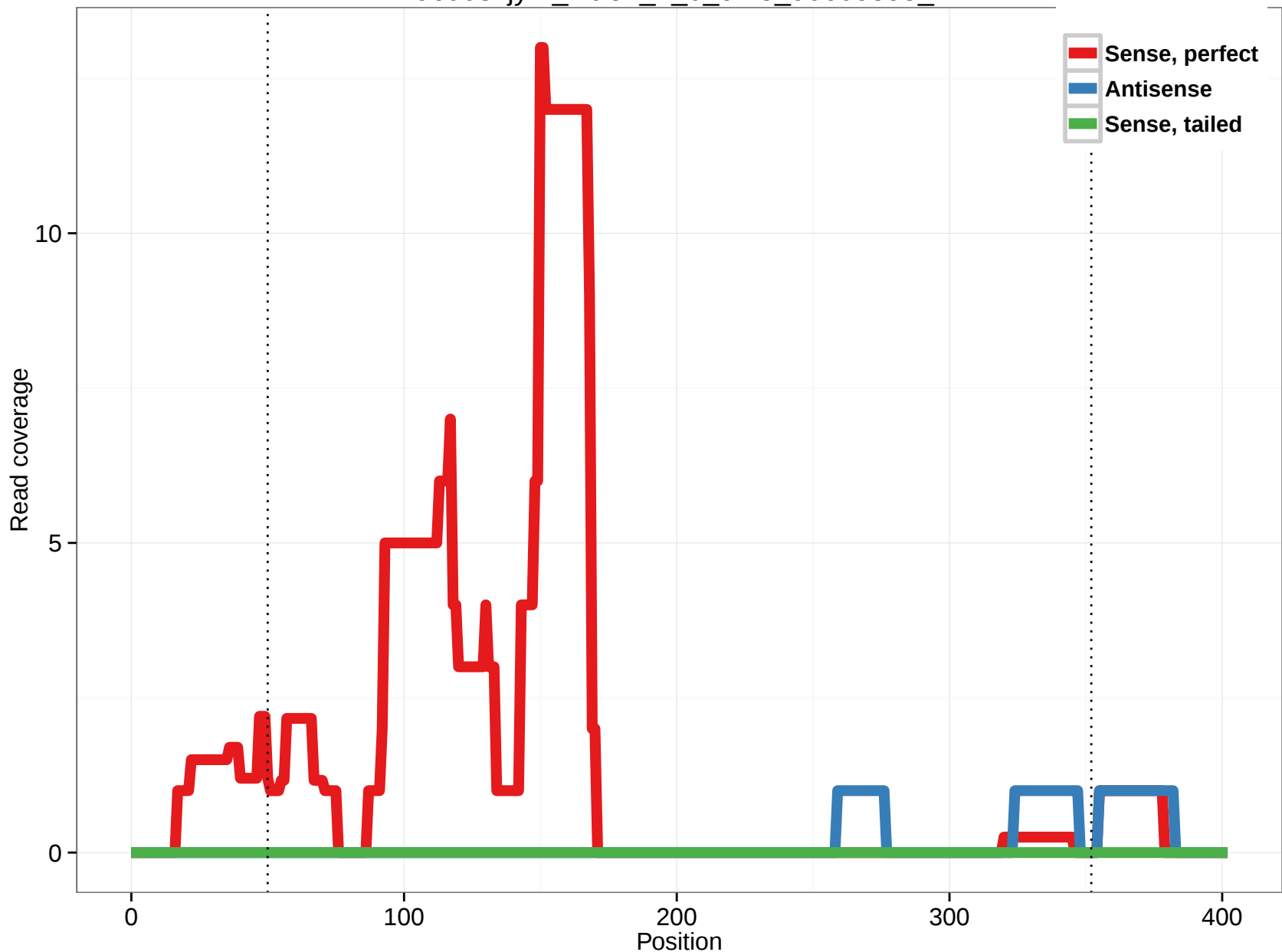
uc003kky.1_intron_1_0_chr5_90609595_r
