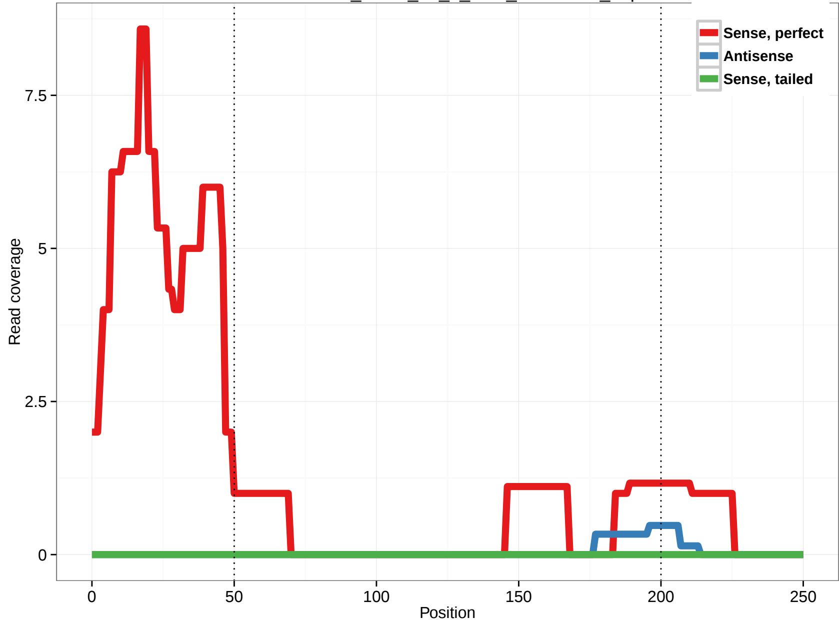
uc003kbn.1_intron_14_0_chr5_70798619_f.5p
