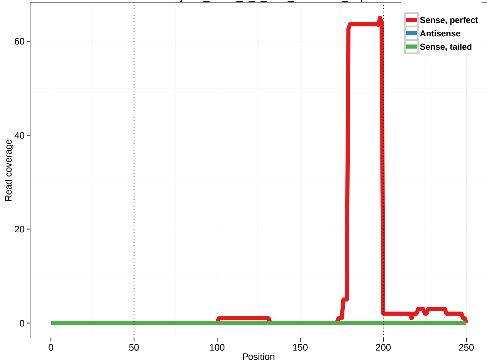
uc003joz.2_intron_2_0_chr5_52397340_r.3p
