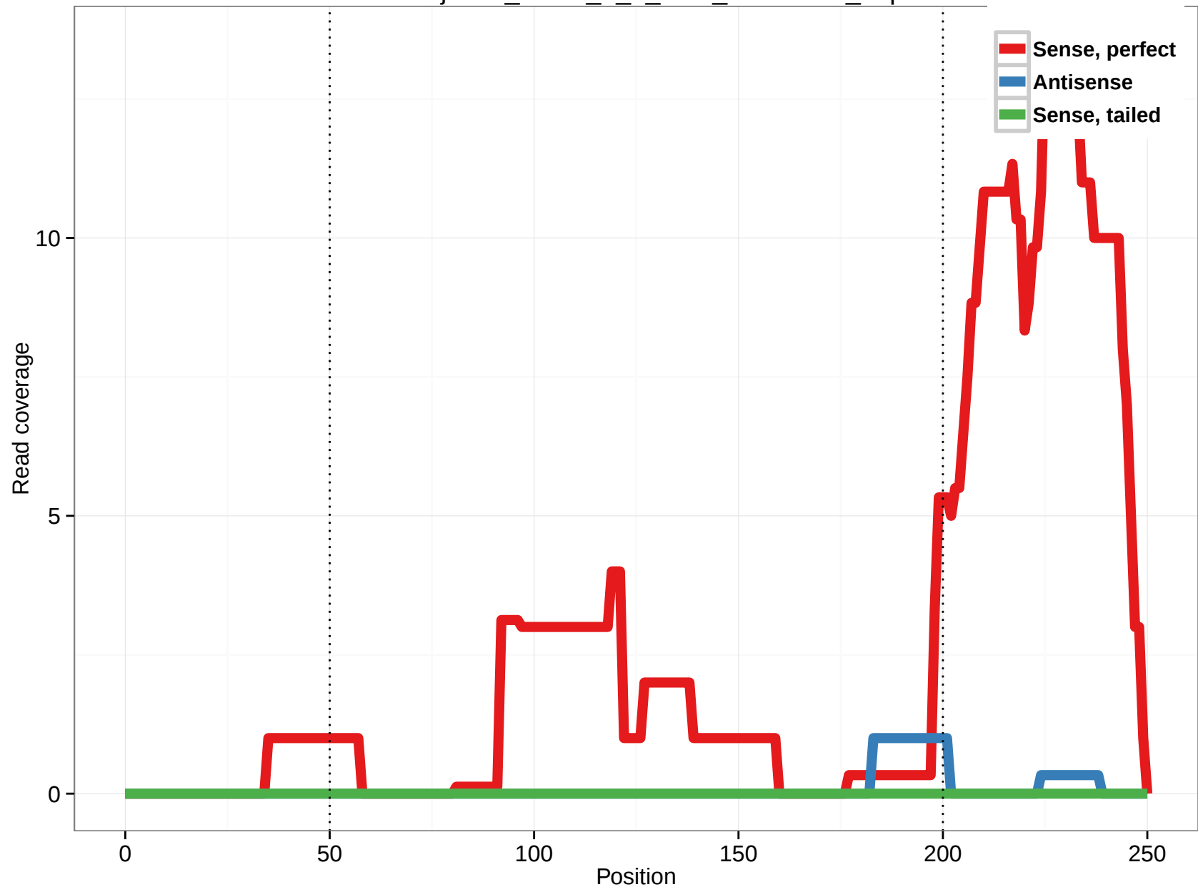
uc003jmo.2_intron_1_0_chr5_41907945_f.3p
