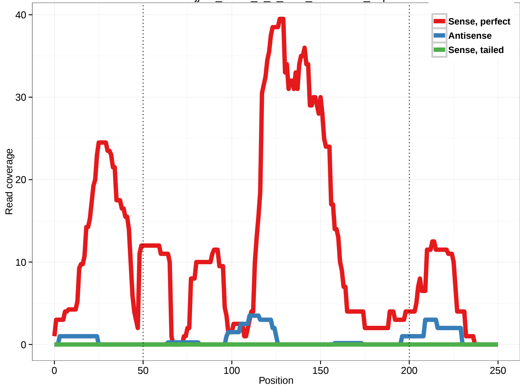
uc003jjb.2_intron_0_0_chr5_34930022_f.5p
