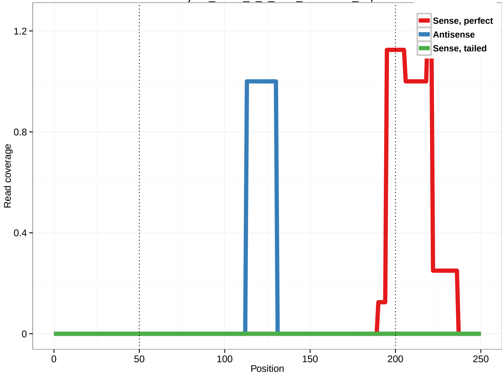
uc003jiu.2_intron_8_0_chr5_34880414_f.3p
