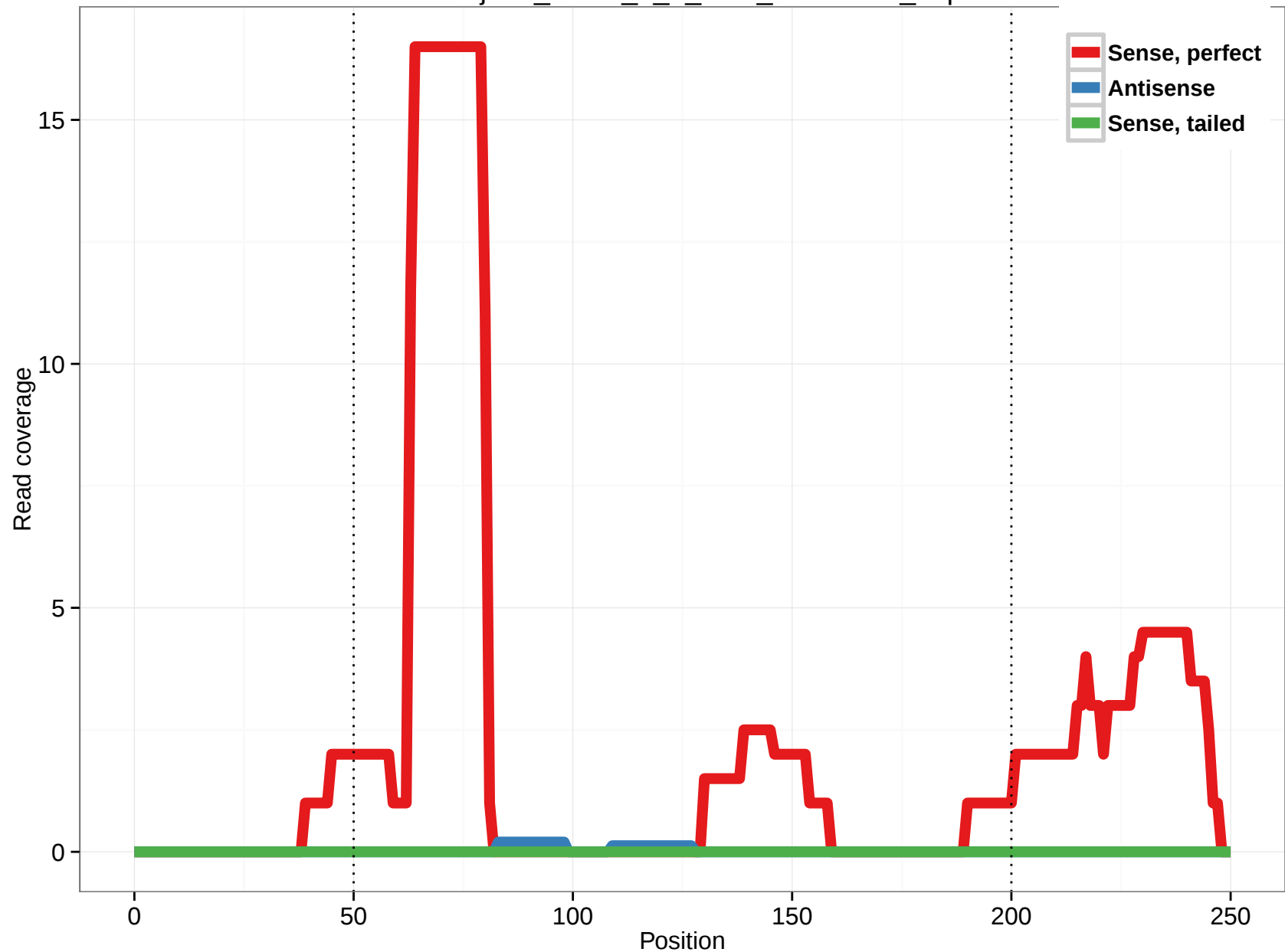
uc003jet.1_intron_9_0_chr5_10397457_f.3p
