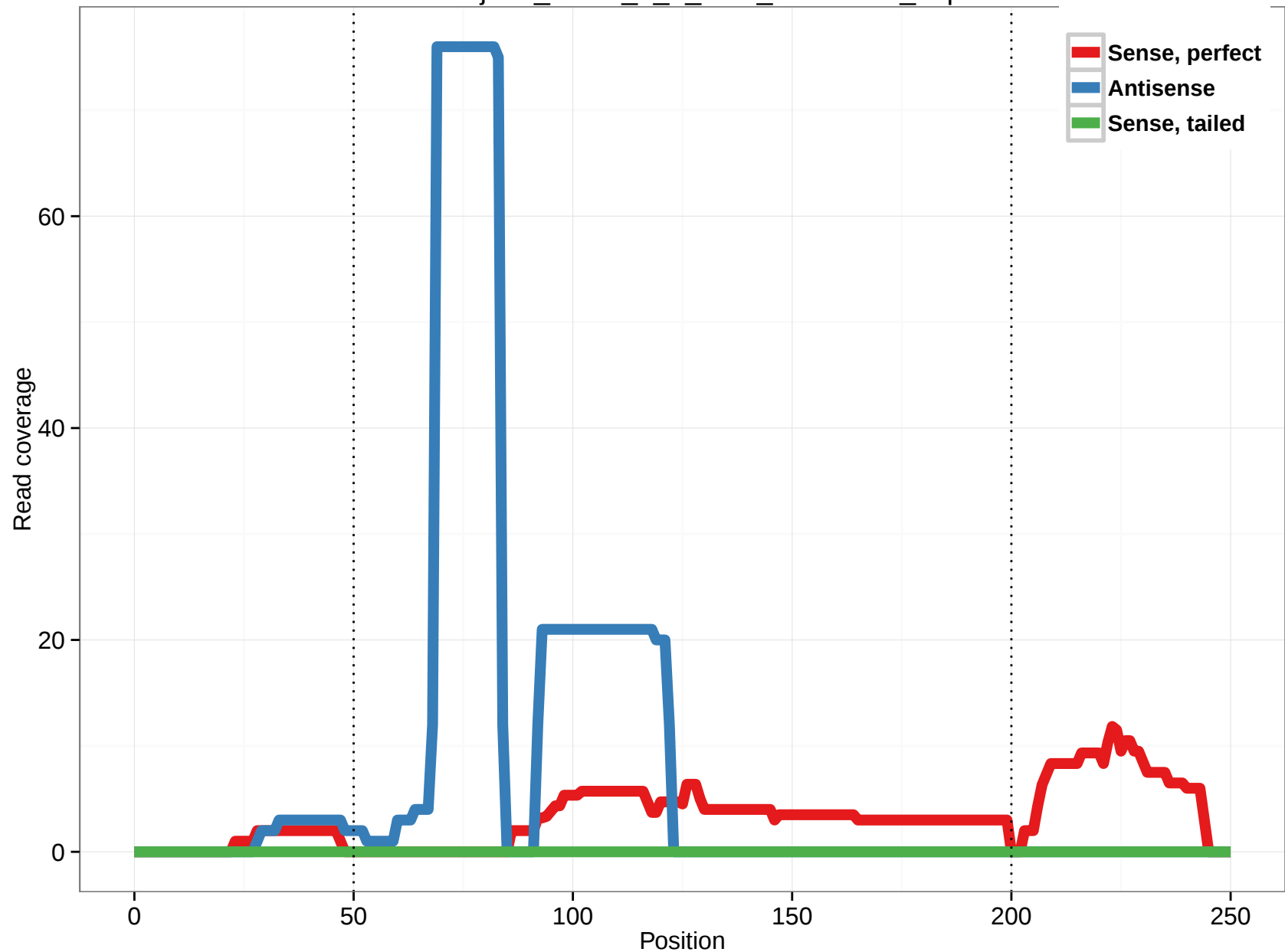
uc003jet.1_intron_5_0_chr5_10390613_f.3p
