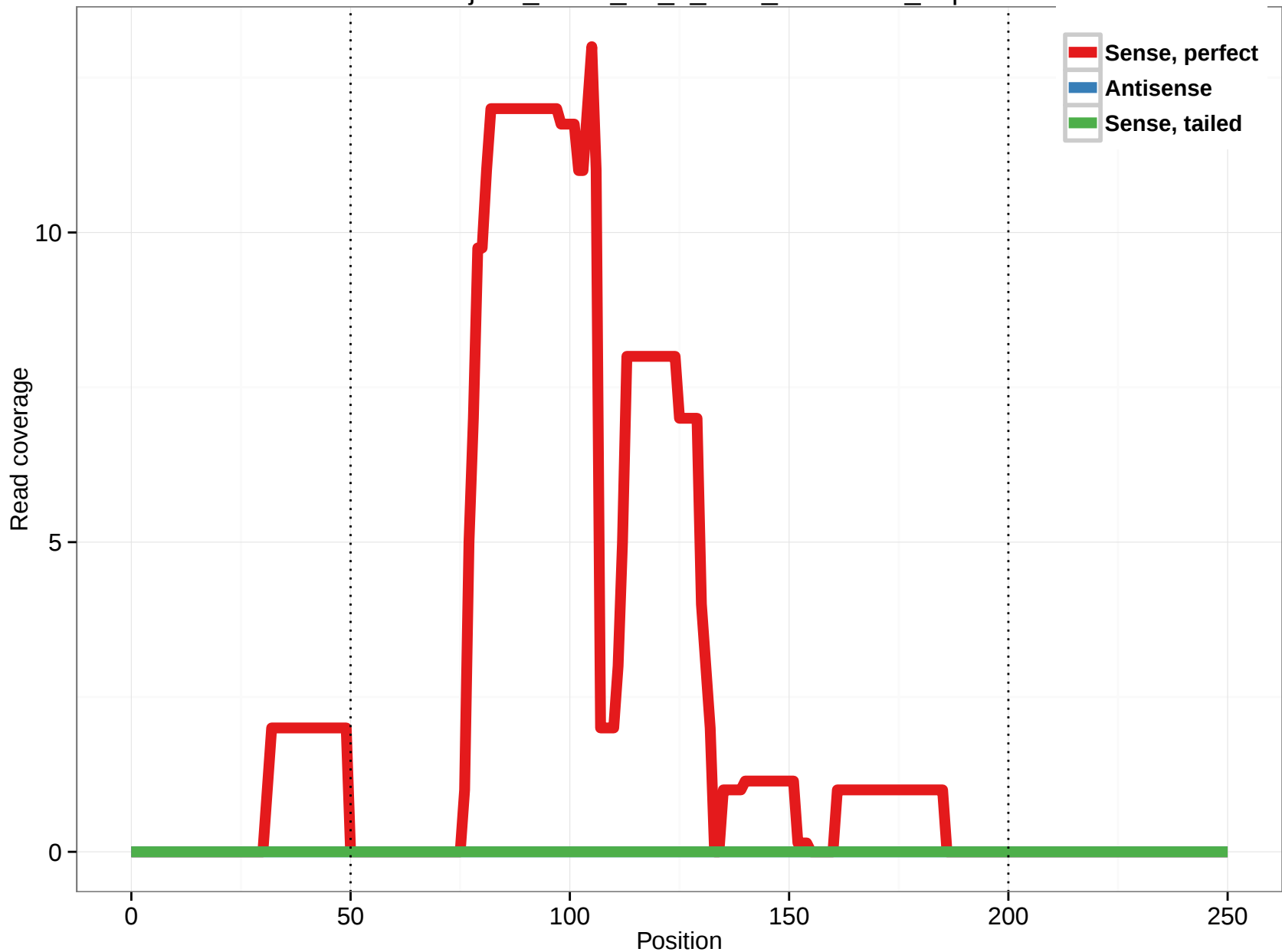
uc003jet.1_intron_18_0_chr5_10411650_f.5p
