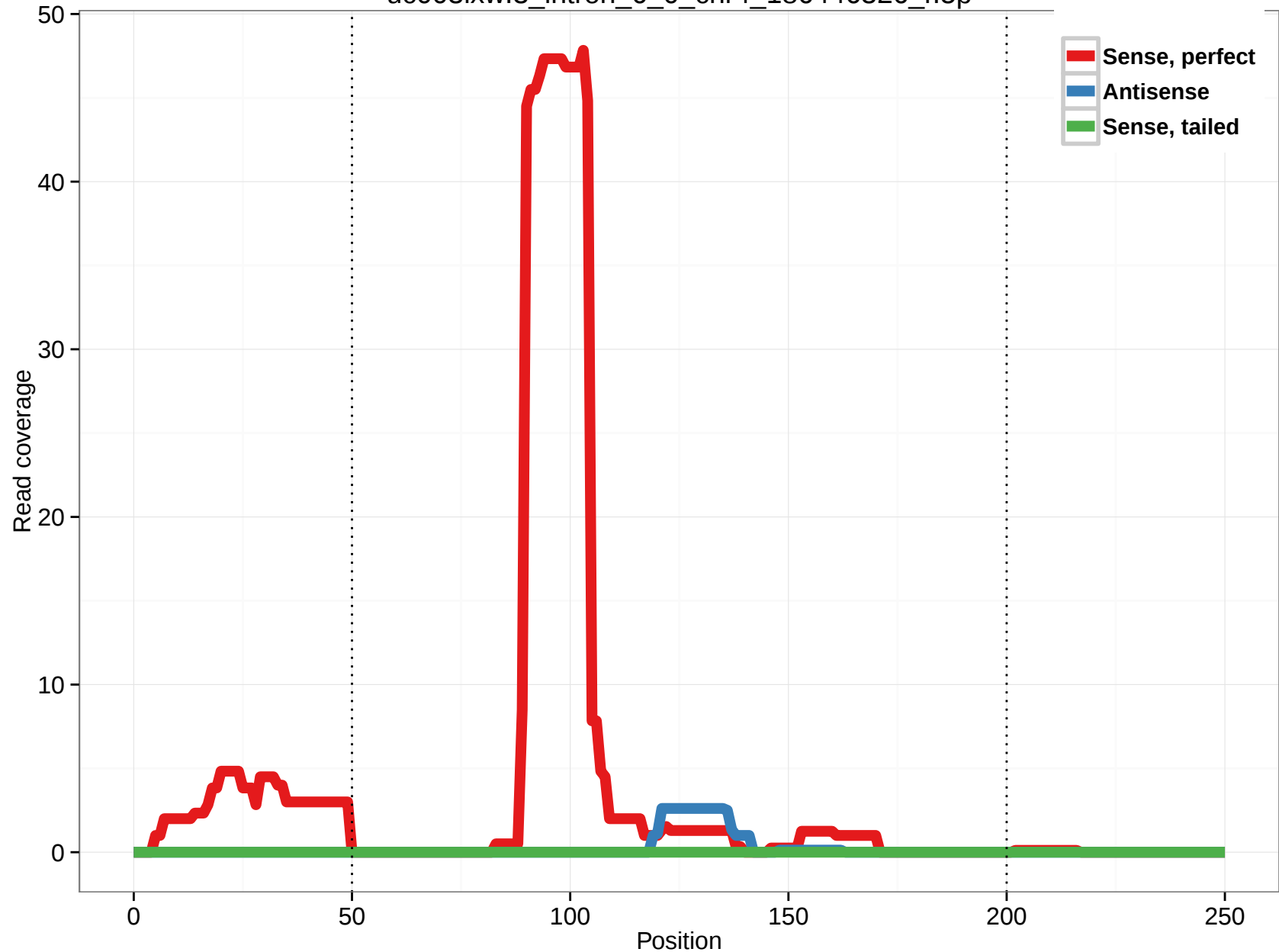
uc003ixw.3_intron_6_0_chr4_186446326_r.5p
