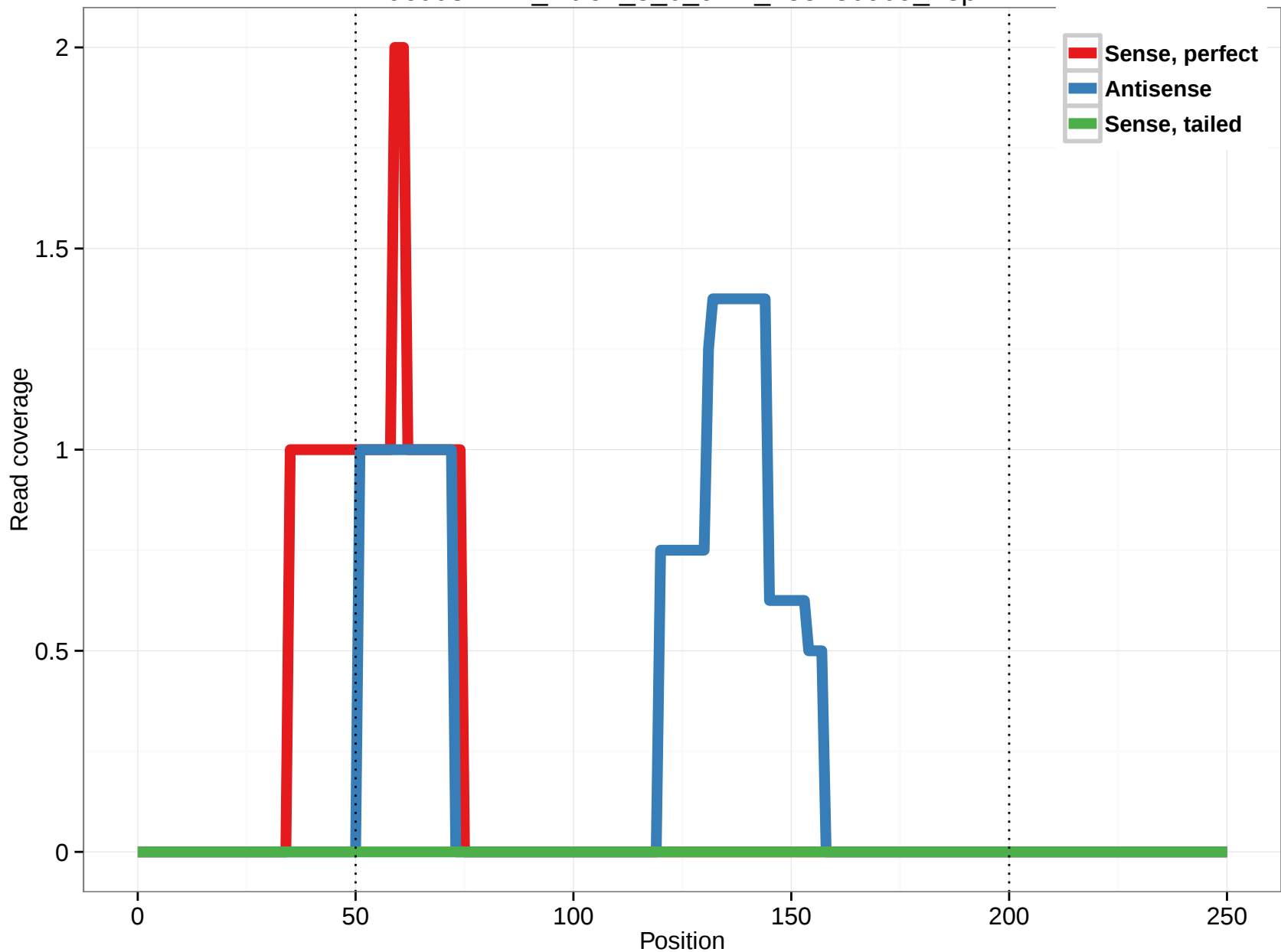
uc003inw.2_intron_5_0_chr4_155180909_r.3p
