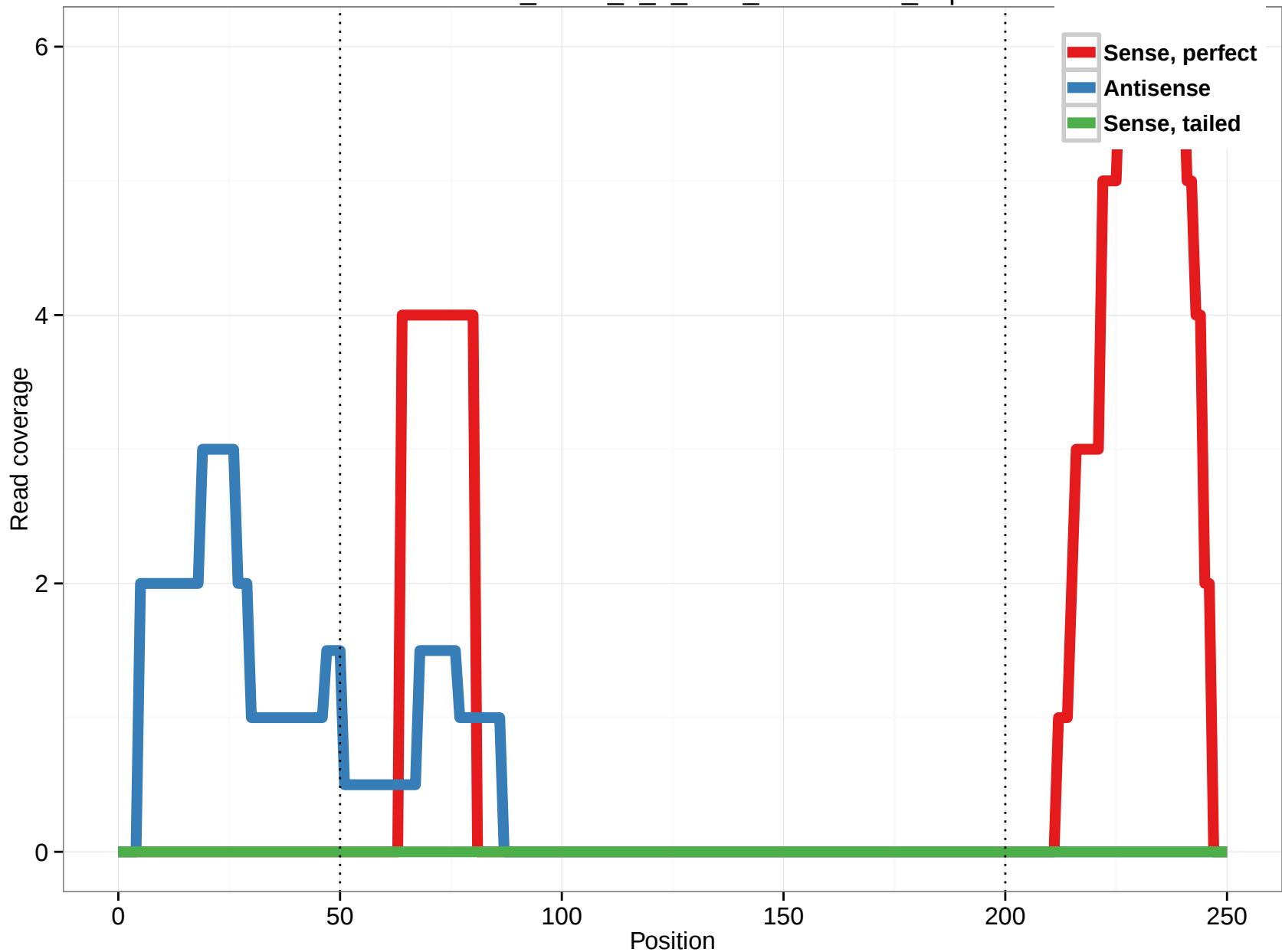
uc003ihu.1_intron_3_0_chr4_140262224_f.3p
