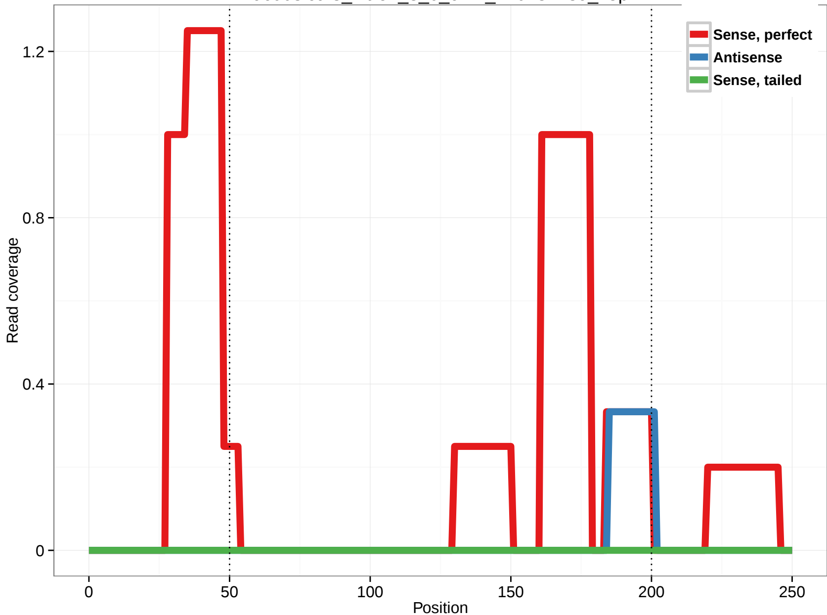
uc003icu.3_intron_8_0_chr4_120187489_f.5p
