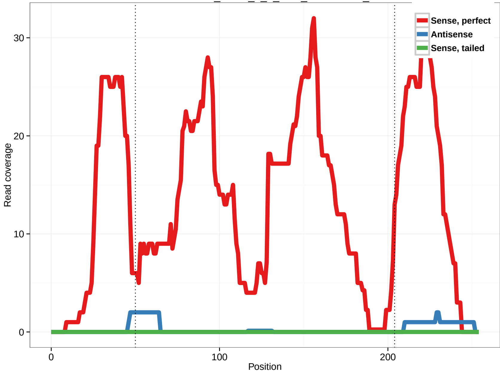
uc003hzz.2_intron_3_0_chr4_111119524_r
