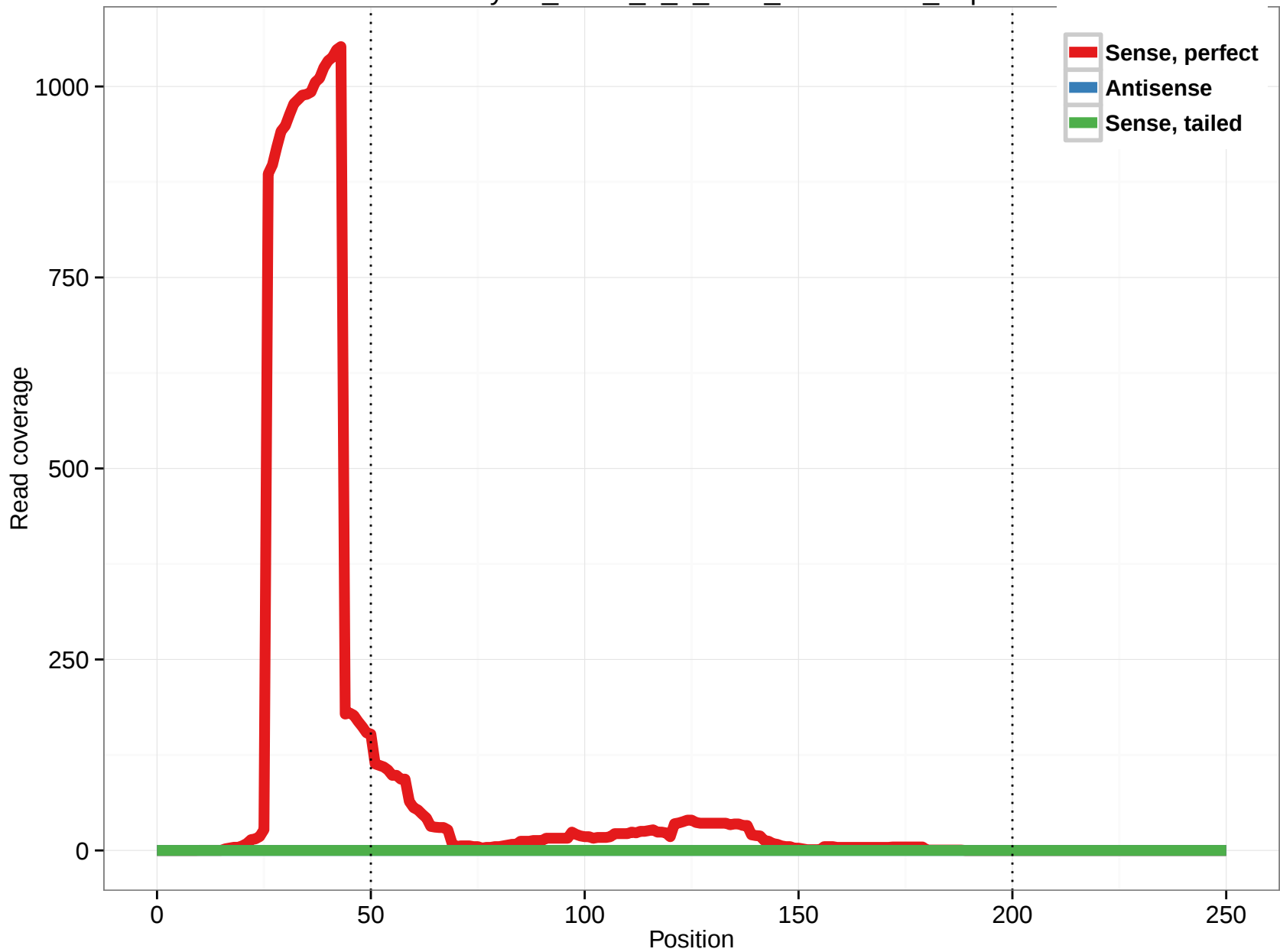
uc003hyz.2_intron_0_0_chr4_109541757_f.5p
