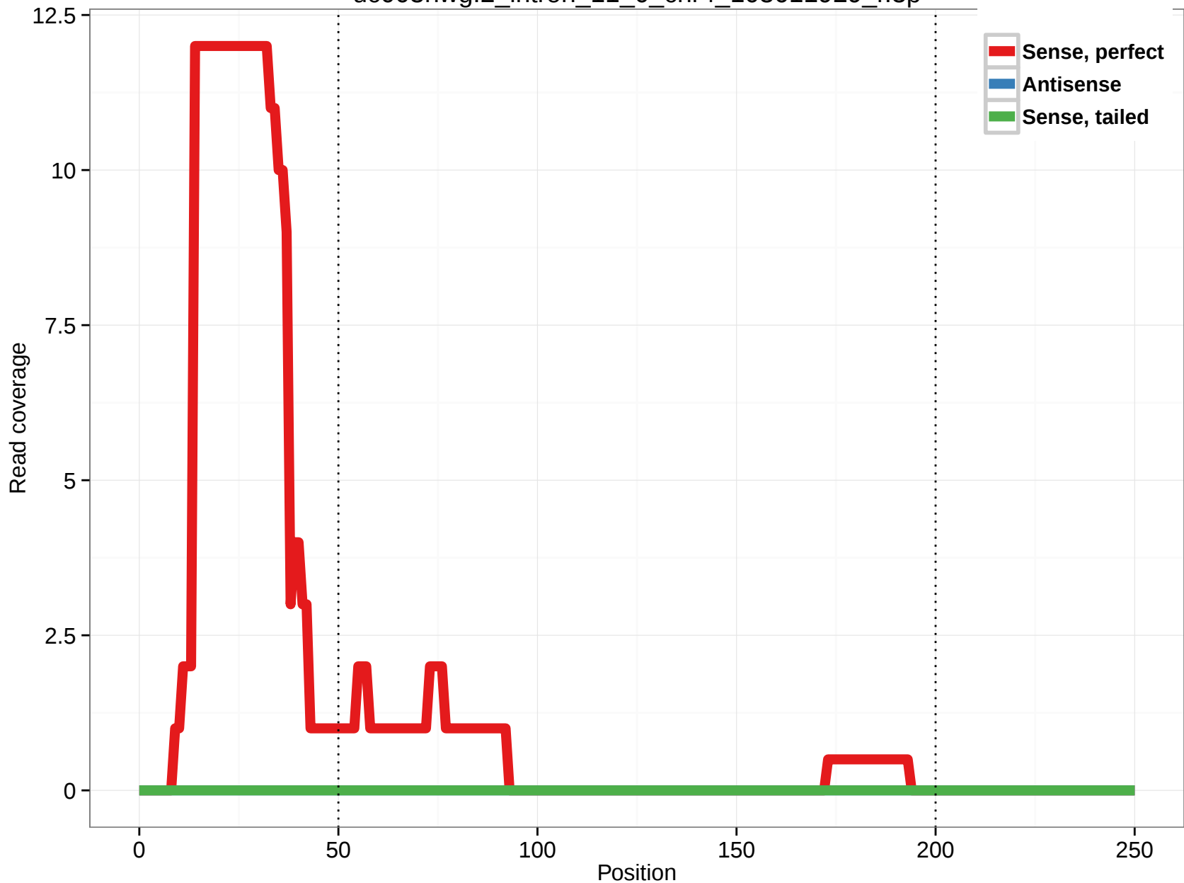
uc003hwg.2_intron_11_0_chr4_103611929_r.3p
