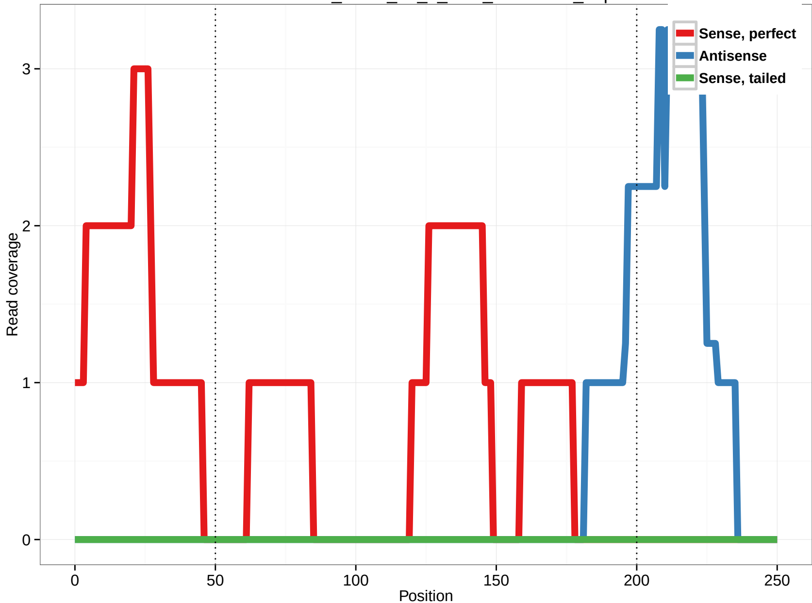
uc003hse.1_intron_17_0_chr4_89772335_r.5p
